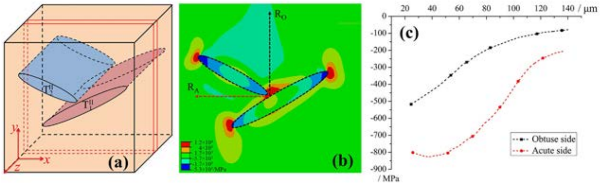
Fig. 5. (a) Schematic of the FEM model. (b) Resolved shear stress fields associated with twin variants T_1^I and T_1^II in the matrix. (c) The variation of the resolved shear stress (MPa, in the vertical axis) along two directions R_0 and R_A ( \mu\text{m} , in the horizontal axis). The resolved shear stress is caused by the back-stress due to the TT junction.
