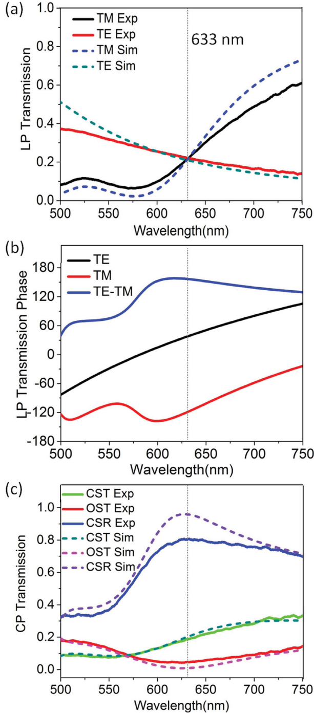
Figure 3. (a) The measured and simulated transmission spectra through the linear grating patterns under linear polarization basis. (b) The simulated transmission phase shifts under linear polarization basis. (c) The measured and simulated converted spin transmission (CST) spectra and original spin transmission (OST) spectra under circular polarization basis, as well as converted spin ratio (CSR).
