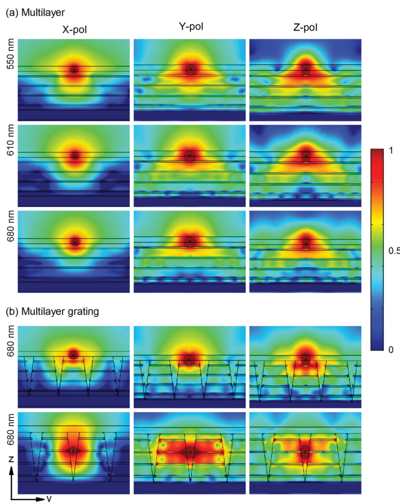
Figure 4. Simulated electric field magnitude distribution of QDs with emission wavelengths of 550, 610, and 680 nm on top of a multilayer (a) and at 680 nm on and inside a multilayer grating (b). Three columns of electric field distributions are from dipole emission with x polarization (X-pol), y polarization (Y-pol), and z polarization (Z-pol), respectively.
