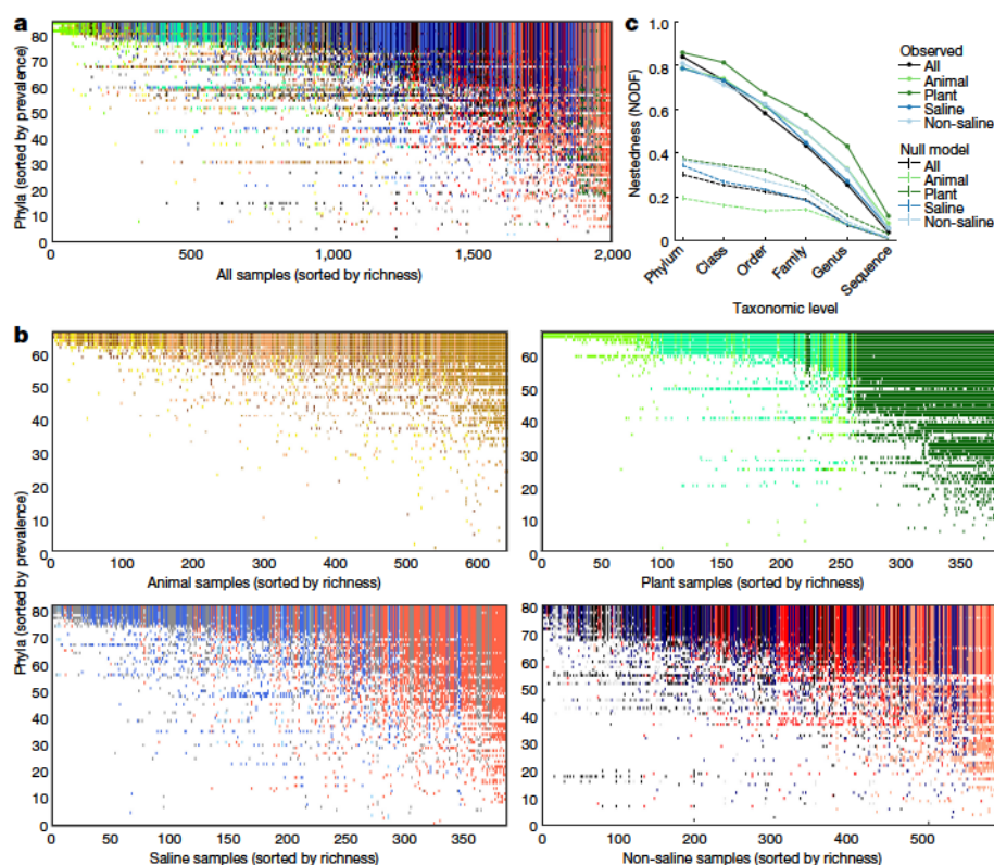
Figure 3 | Nestedness of community composition. a, Presence-absence of phyla across samples, with phyla (rows) sorted by prevalence and samples (columns) sorted by richness. Shown is a subset of the EMP consisting of n = 2,000 biologically independent samples with even representation across environments and studies. With increasing sample richness (left to right), phyla tended to be gained but not lost ( P < 0.0001 versus null model; NODF (nestedness measure based on overlap and decreasing fills) statistic and 95% confidence interval = 0.841 \pm 0.018 ). b, As in a but separated into non-saline, saline, animal, and plant environments ( P < 0.0001 , respective NODF = 0.811 \pm 0.013 , 0.787 \pm 0.015 , 0.788 \pm 0.018 and 0.860 \pm 0.021 ). c, Nestedness as a function of taxonomic level, from phylum to tag sequence, across all samples and within environment types. Also shown are median null model NODF scores ( \pm s.d.). NODF measures the average fraction of taxa from less diverse communities that occur in more diverse communities. All environments at all taxonomic levels were more nested than expected randomly, with nestedness higher at higher taxonomic levels (for example, phyla).
