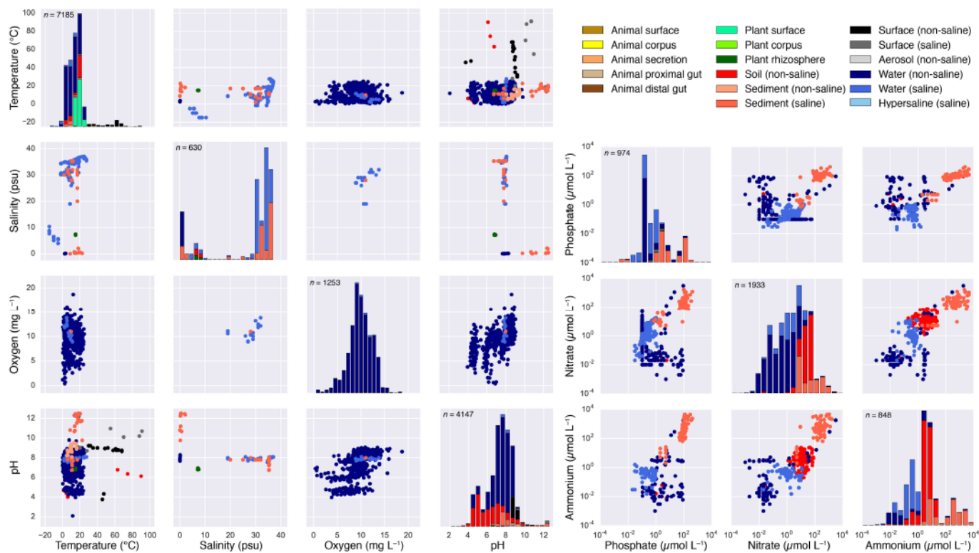
Extended Data Figure 1 | Physicochemical properties of the EMP samples. Pairwise scatter plots of available physicochemical metadata are shown for temperature, salinity, oxygen, and pH, and for phosphate, nitrate, and ammonium. Histograms for each factor are also shown; the number ( n ) of samples having data for each factor is provided at the
