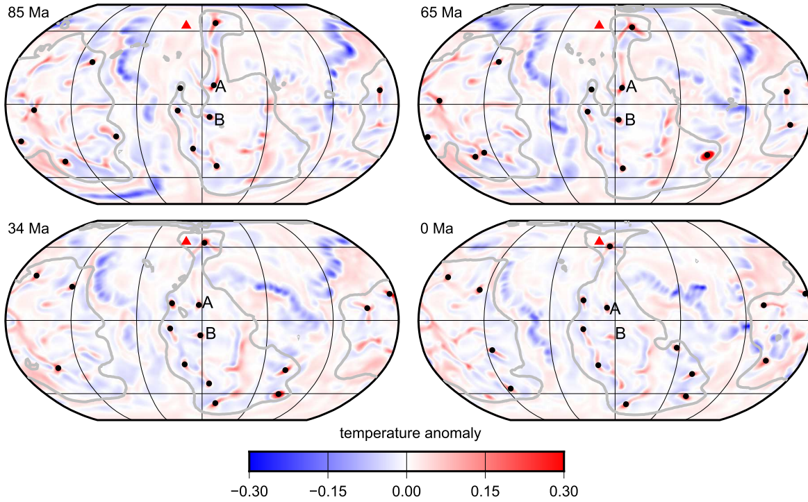
Fig. 5. Snapshots of temperature anomaly at 1500 km depth for Case 2. The gray contours show the edges of thermochemical piles at 2800 km depth. The black dots show locations of strong plumes whose maximum temperature anomaly is higher than 0.2. The symbols A and B show locations of plumes which are discussed in the text. The red triangles show the location of the Iceland. The figures are centered at longitude = 0°. (For interpretation of the references to color in this figure legend, the reader is referred to the web version of this article.)
