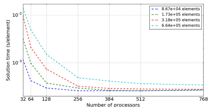
Fig. 15. Moltres extra-node strong scaling efficiency for various problem size, for n_{nodes} \in [1, 24] .
