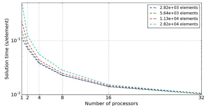
Fig. 14. Moltres intra-node strong scaling efficiency for various problem sizes, for n_{cores} \in [1, 32] .
