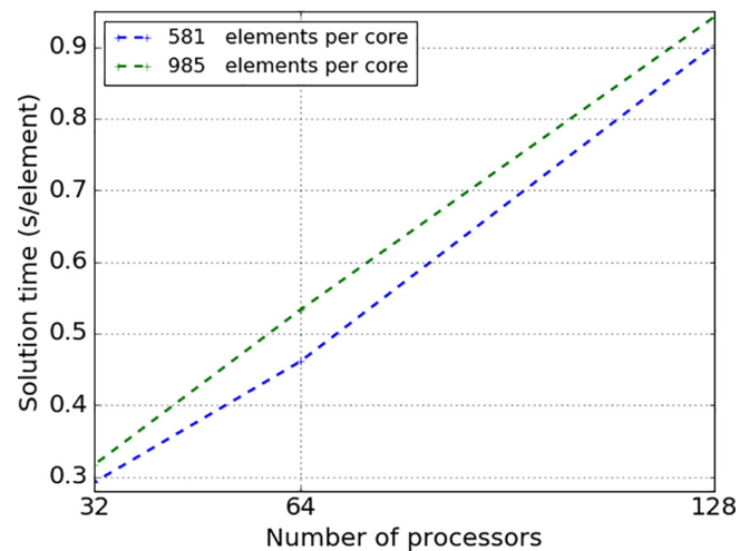
Fig. 17. Weak scaling performance of Moltres on Blue Waters, in seconds per element vs. number of processors, for a constant number of elements per processor, for and n_{cores} \in [32, 128] .
