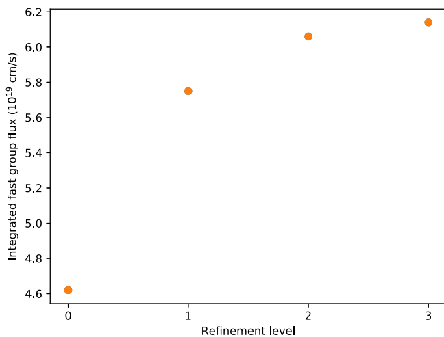
Fig. 2. Plot of the integrated fast group flux as the mesh in isotropically refined.
