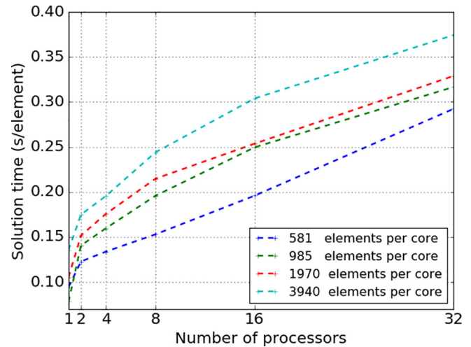
Fig. 16. Weak scaling performance of Moltres on Blue Waters, in seconds per element vs. number of processors, for a constant number of elements per processor, and n_{cores} \in [1, 32] .
