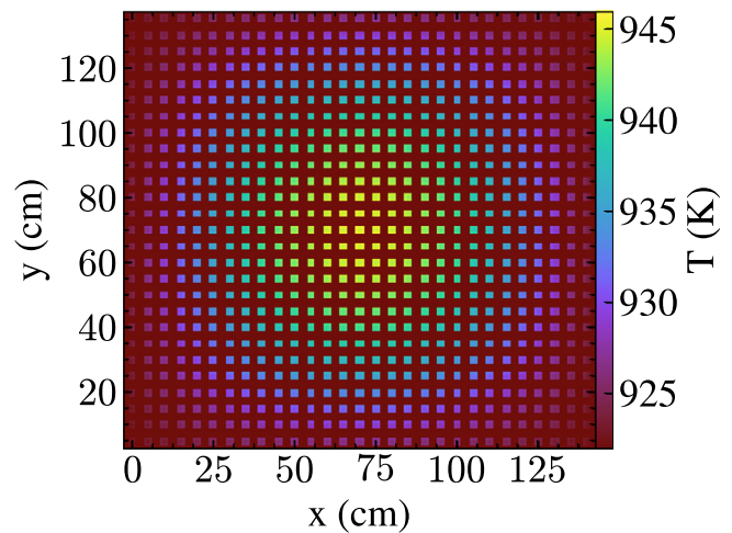
Fig. 10. Temperature at the reactor outlet for 3D MSRE-like model.
