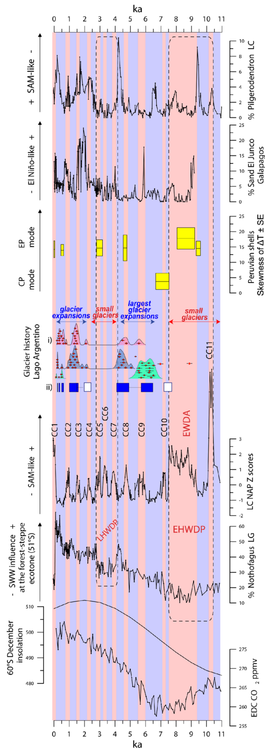
Figure 3. Southern Hemisphere climate comparisons. We compare the last 11,000 years of the standardized Lago Cipreses Non Arboreal Pollen curve (LC NAP) (D) with the the EPICA Dome C record of atmospheric 13 CO 2 (A); the December insolation at 60°S (B); the % Nothofagus abundance in Lago Guanaco (LG) 21 (C), a proxy for precipitation of SWW origin in the Torres del Paine area, downwind from LC; a summary of the cosmogenic and radiocarbon constraints (E) on Patagonian glacier history in the Lago Argentino sector 45,46 , we show 10 Be ages ( \pm 1\sigma ), summed probability density plots of all the ages (i.e., camel humps), and mean moraine ages (blue and white rectangles) based on published 10 Be and 14 C data. The 'camel humps' essentially reflect times of moraine formation and hence glacier expansion relative to today. (F) Shows the skewness of delta temperature ( \pm standard error) from Peruvian shells interpreted 5 as a proxy for Eastern Pacific (EP, values > 0 ) or Central Pacific (CP, values < 0 ) modes in El Niño regime; (G) the % sand record from lake El Junco in Galapagos 38 (G), a proxy for El Niño activity in the eastern equatorial Pacific; and (H) the % Pilgerodendron abundance in the LC record in its original units and standardized units in the z-scored secondary scale, which we
