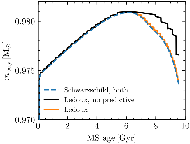
Figure 9. Mass coordinate m_{\text{bdy}} of the lower boundary of the envelope convection region plotted as a function of MS age, for the 1 M_{\odot} stellar model discussed in Section 2.5. Different line styles/colors show the separate runs described in the text.
