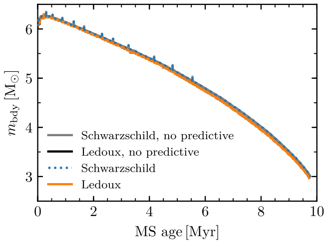
Figure 3. Mass coordinate m_{\text{bdy}} of the convective-core boundary as a function of MS age, for the 16 M_{\odot} stellar model discussed in Section 2.3. Different line styles/colors show the separate runs described in the text.
