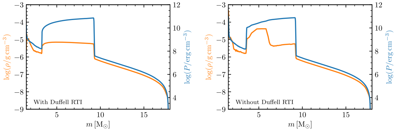
Figure 29. Density (left y-axis, orange curves) and pressure (right y-axis, blue curves) for MESA models with the Duffell RTI (left panel) and without any RTI effects (right panel) at a time when the forward shock is approximately halfway through the star. The animated figure shows the time evolution of these and other quantities for each case.
