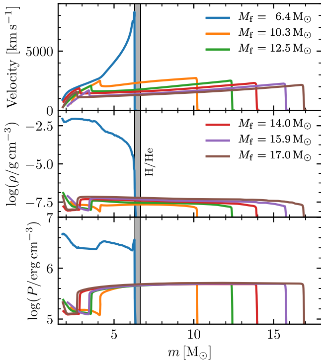
Figure 46. Models of M_{\text{ZAMS}} = 17 M_{\odot} stars (case “stripped”) that have experienced a range of stripping. The density, velocity, and pressure profiles are shown at the time of handoff from MESA to STELLA, very close to shock breakout. The gray band shows the range of locations of the H/He boundary at the time of explosion.
