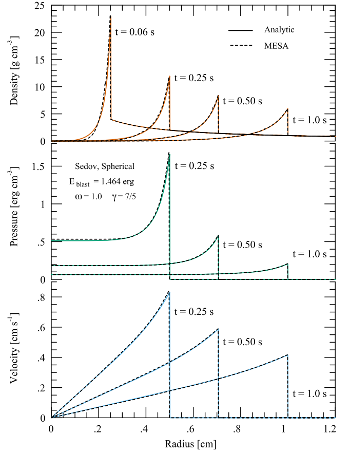
Figure 20. Sedov blast wave density, pressure, and velocity profiles at the labeled times. The analytic (black) and MESA (colored) curves show solutions for a shock propagating down a \rho = \rho_0 r^{-1} density profile with an adiabatic index \gamma = 7/5 . Deviations from the analytic solutions are \lesssim 2\% .
