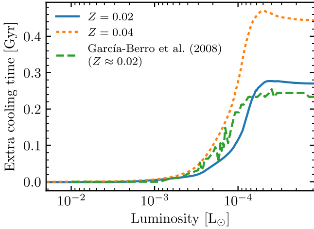
Figure 18. Extra cooling time required to reach a given luminosity for 0.6 M_{\odot} WD models including heating from ^{22}\text{Ne} settling, relative to models ignoring this heating. For comparison, we also show a result from García-Berro et al. (2008) for a 0.6 M_{\odot} WD with an oxygen-dominated core composition. Figure 57 shows the same quantity including other physical processes such as crystallization for the same Z = 0.02 WD model shown here.
