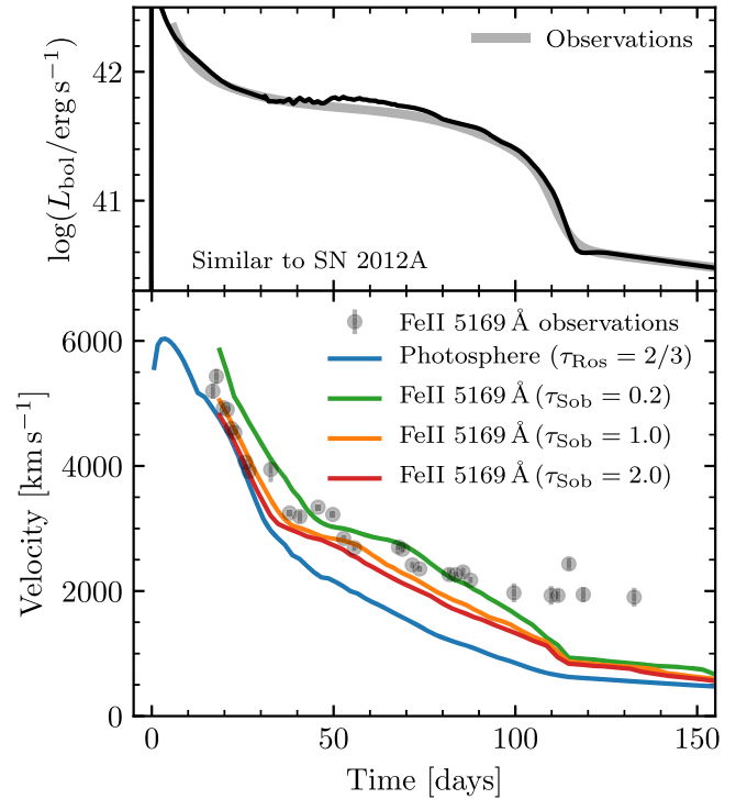
Figure 36. Comparison of different definitions of velocity for a model (12A) similar to SN 2012A. The upper panel shows the data and the model for the bolometric luminosity. The lower panel shows the velocity of a few different locations depending on the Sobolev optical depth in the Fe II line.
