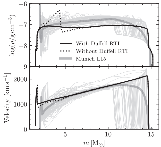
Figure 28. Comparison of density (upper panel) and velocity (lower panel) profiles. The solid black line shows the MESA model using the Duffell RTI capabilities documented here with D_R = 3 ; the dotted black line shows the same model run without the effects of the RTI. The thick gray lines show the 1D shell averages of the Munich model, while the fainter gray lines show the Munich model densities and velocities at different angles.
