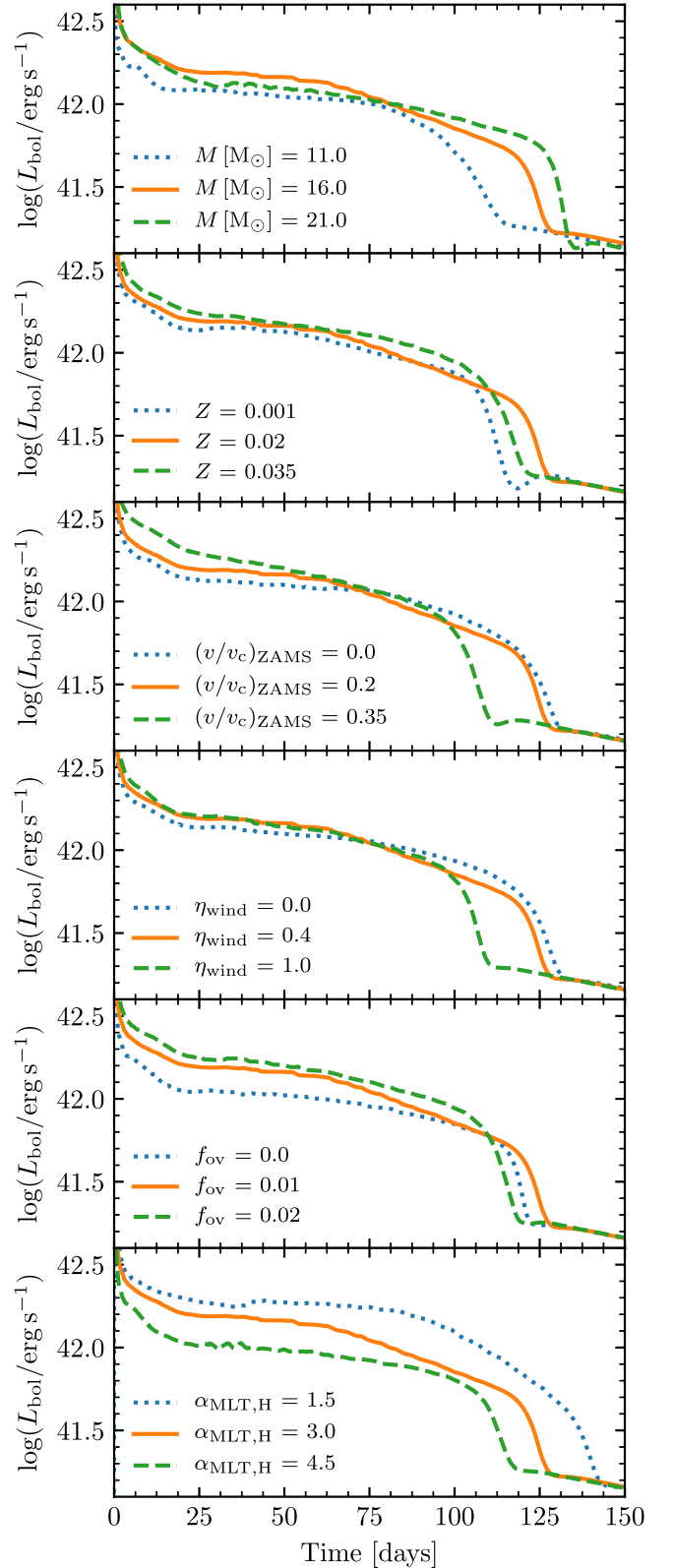
Figure 39. Effect of single-parameter variations of the progenitor std_16. The upper three panels vary initial properties of the star; the lower three vary modeling assumptions during evolution to core collapse.
