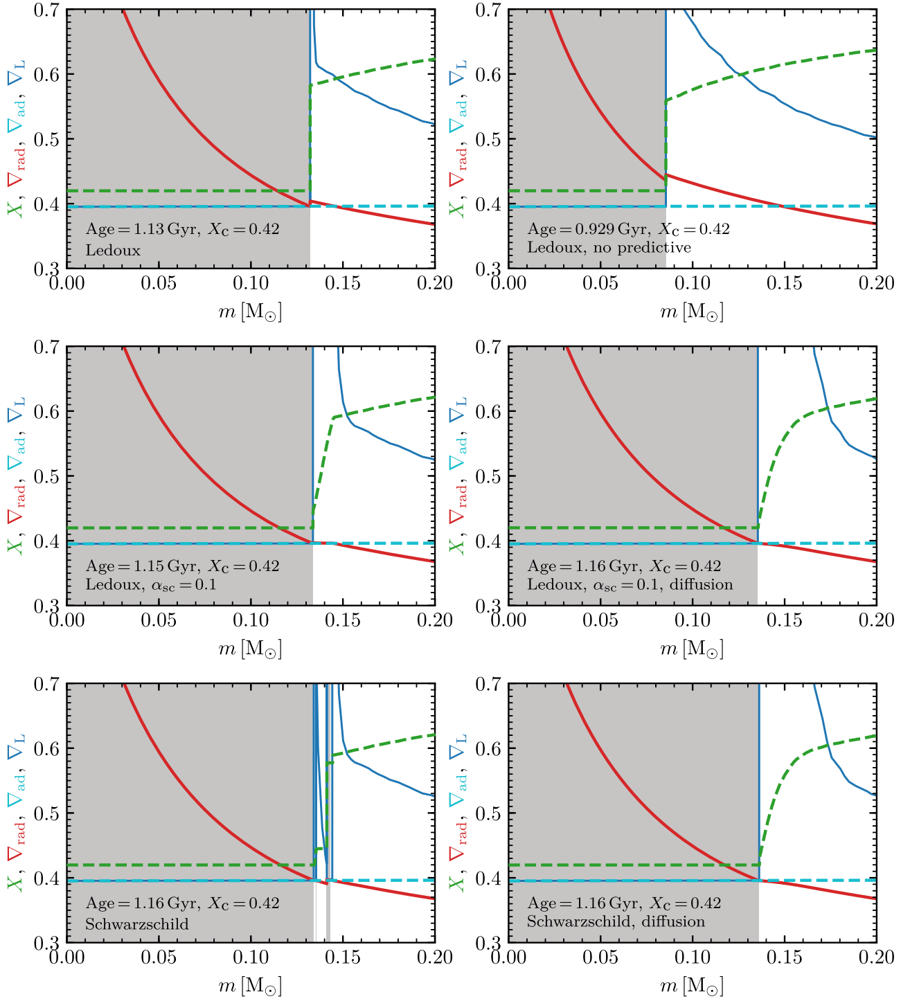
Figure 2. Profiles of \nabla_{\text{rad}} , \nabla_{\text{ad}} , \nabla_L , and X as a function of mass coordinate, in the inner part of the 1.5 M_{\odot} stellar model at X_c = 0.42 . The panels show the separate runs described in the text. Gray shading indicates regions undergoing convection. Unless otherwise indicated, all models used predictive mixing.
