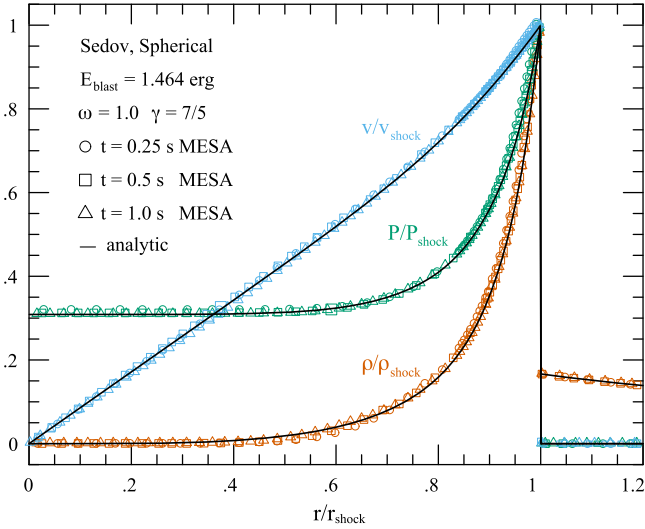
Figure 21. Sedov blast wave self-similarity of the analytic (black curves) and MESA (colored symbols) solutions. Scaled velocity v/v_{\text{shock}} , pressure P/P_{\text{shock}} , and density \rho/\rho_{\text{shock}} profiles for a shock propagating down a \rho = \rho_0 r^{-1} density profile at the three different times are overlaid. Symbols for each epoch mark cell locations. Deviations from the analytic self-similar solutions are \lesssim 2\% .
