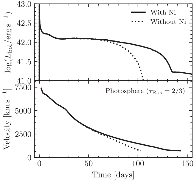
Figure 33. Light curves and velocities for a model similar to SN 1999em with \approx 0.04 M_{\odot} ^{56}\text{Ni} and without ^{56}\text{Ni} . The main effect of the radioactive decay is to prolong the plateau.
