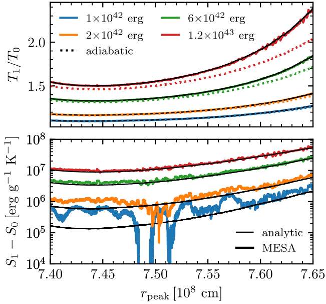
Figure 26. Comparison of the MESA calculation (colored lines) to the expectations of shock theory (thin black lines) for the temperature increase (upper) and entropy increase (lower) for different energies injected. Colored dotted lines in the upper plot indicate the temperature change for a purely adiabatic compression.
