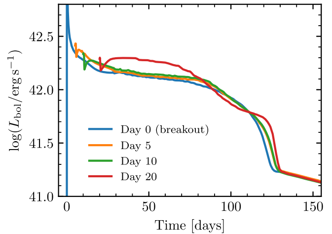
Figure 31. Bolometric light curves for Type IIP SNe obtained where the transition between MESA and STELLA has been done at different times relative to shock breakout. Performing the handoff just before breakout (blue curve, day 0) is the recommended choice.
