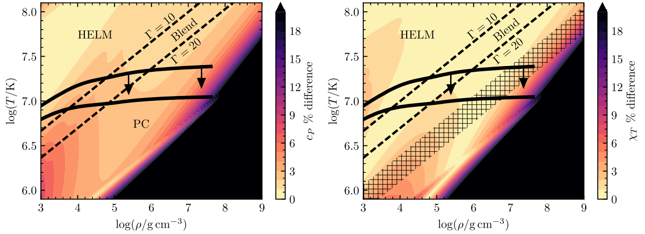
Figure 59. Percent difference between HELM and PC EOS for c_P (left) and \chi_T (right). Dashed lines show the EOS blending boundaries for 10 \leq \Gamma \leq 20 , and the hatched region in the right panel shows the previous default blending range 40 \leq \Gamma \leq 80 . In the new blending region, the EOSs disagree by only a few percent for these quantities.
