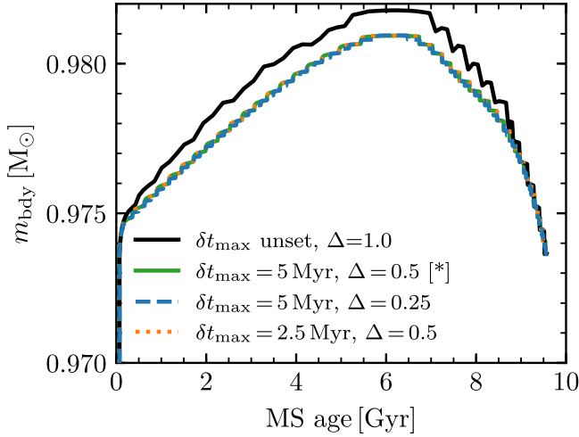
Figure 11. Mass coordinate m_{\text{bdy}} of the lower boundary of the envelope convection region plotted as a function of MS age, for the 1 M_{\odot} stellar model. Different line styles/colors show the separate runs with alternative time step ( \delta t_{\text{max}} ) and mesh resolution ( \Delta ) choices. The choices adopted in Section 2.5 are marked with an asterisk [*].
