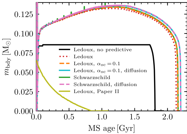
Figure 1. Mass coordinate m_{\text{bdy}} of the convective-core boundary plotted as a function of MS age, for the 1.5 M_{\odot} stellar model discussed in Section 2.2. Different line styles/colors show the separate runs described in the text.
