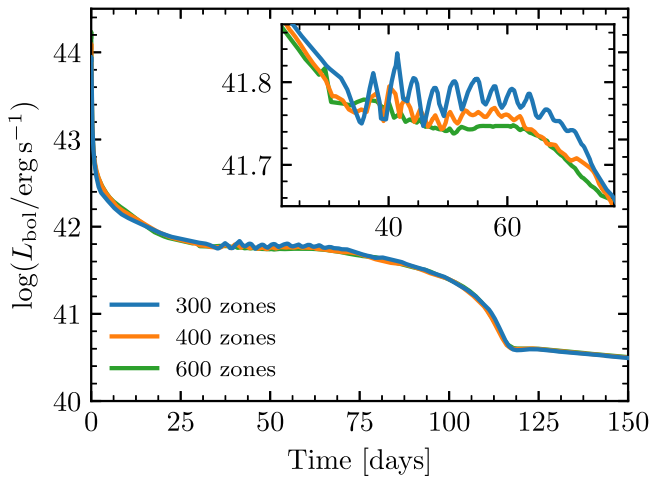
Figure 30. Effect of number of STELLA zones on a model (12A) similar to SN 2012A. The inset zooms in on the region of the plateau that exhibits numerical oscillations. A small increase in the number of zones significantly reduces this artifact, and doubling the number of zones almost completely removes it.
