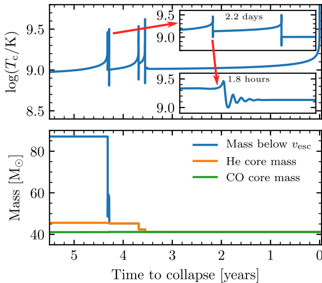
Figure 50. Late-time evolution of an M_{\text{ZAMS}} = 90 M_{\odot} star with metallicity Z = 0.001 undergoing a PPISN. (Upper panel) Evolution of the central temperature showing a zoomed-in region, covering 2.2 days, which contains the first two pulses, as well as an additional zoomed-in region covering 1.8 hr, which shows the first pulse and its ring-down into hydrostatic equilibrium. (Lower panel) Total mass of the star below the escape velocity, He core mass, and CO core mass during pulsations. The animated figure shows the time evolution of these quantities and the interior structure of the star.
