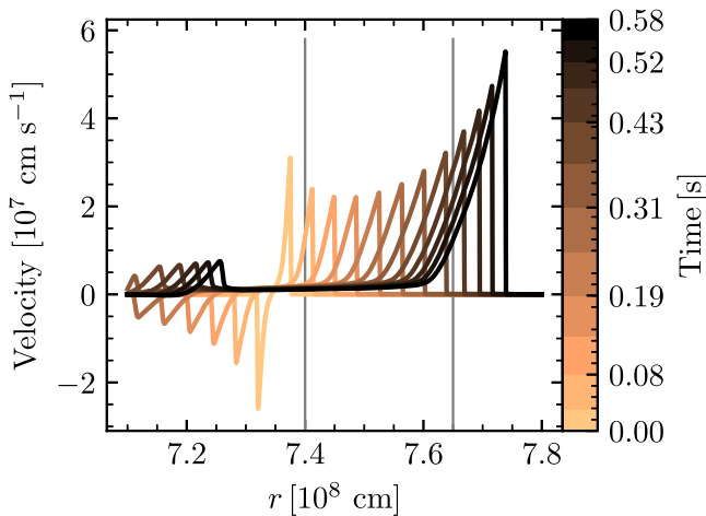
Figure 24. Velocity at different times in the envelope after 6 \times 10^{42} erg has been injected. One shock front travels upward and grows as it enters the outer atmosphere, and another pulse travels downward and reflects off of the inner boundary. The thin gray lines denote the region of study.
