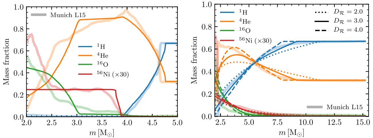
Figure 27. Comparison of abundances in MESA models (thin lines) with 3D shell averages from the Munich L15 model (thick lines). This is a comparison of analogous models at similar times, so the goal is to illustrate qualitative agreement. Left panel: for D_R = 3 , the time when the forward shock is at 4.8 M_\odot and the reverse shock at about 4.0 M_\odot . The MESA ^{56}\text{Ni} curve is the result of artificially inserting ^{56}\text{Ni} in the model at this time. Right panel: the time the forward shock is at 14.7 M_\odot , so near breakout, and for D_R = 2, 3 and 4 .
