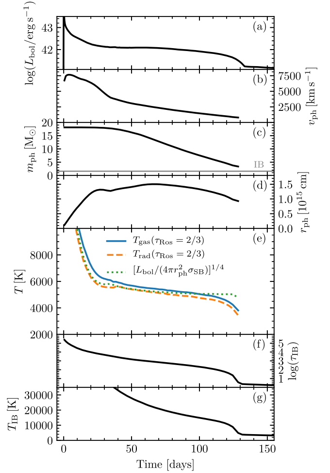
Figure 34. Photosphere and IB properties of a model (99em_19 in Table 3) similar to the Type IIP SN 1999em, as a function of time. From top to bottom, the figure shows the bolometric luminosity, velocity, mass coordinate, and radius coordinate of the photosphere; three temperatures (gas, radiation, and “effective”) at the photosphere; the optical depth to the IB; and the IB temperature. The gray line in panel (c) shows the Lagrangian mass coordinate of the IB.
