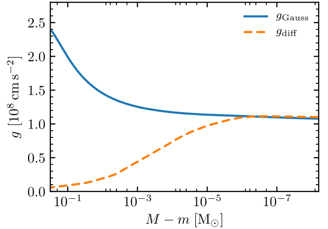
Figure 14. Gravitational acceleration reported by the diffusion routine described in Paper III compared with g_{\text{Gauss}} = Gm/r^2 for a 0.6 M_{\odot} MESA WD model.
