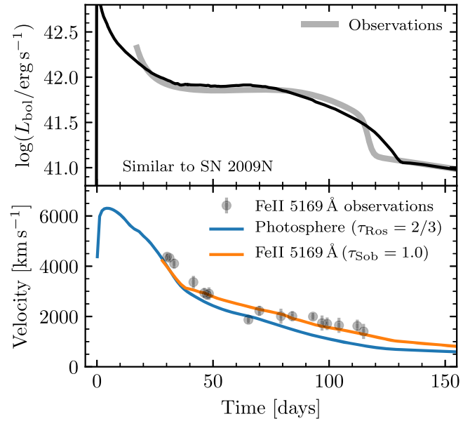
Figure 44. Model (09N) similar to SN 2009N. Further experiments might produce a model with a better match to the drop at the end of the plateau. Alternatively, this model might be a useful start when looking for a match to an observed light curve with a slow decline from the plateau.
