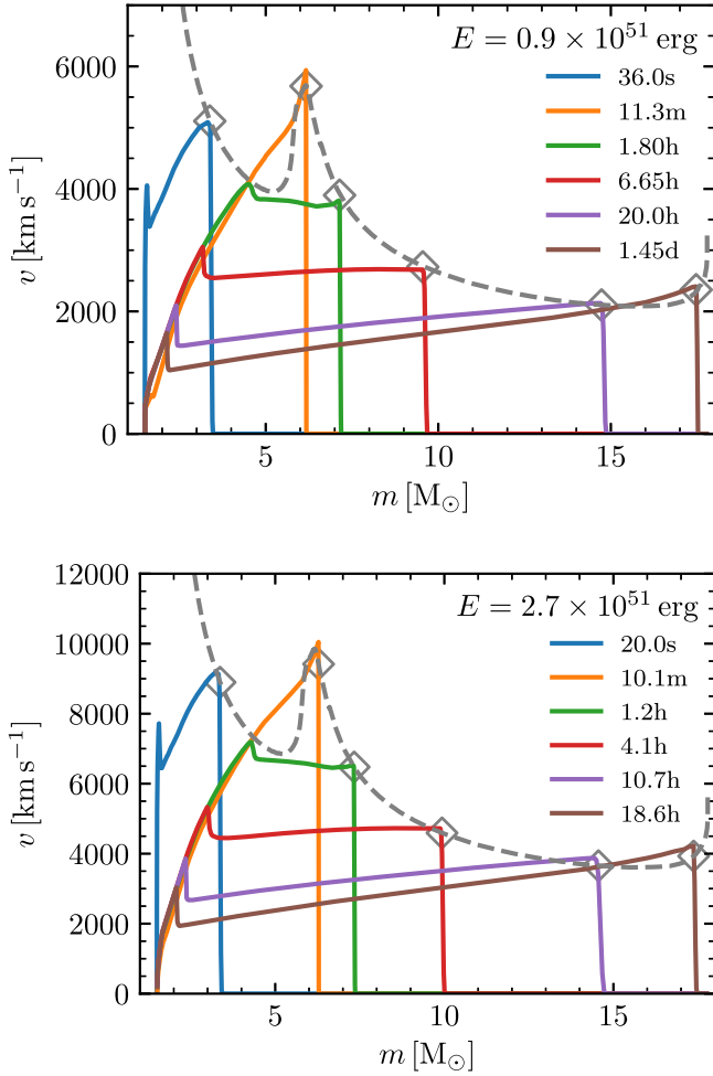
Figure 23. Comparison of MESA with the analytic results of Matzner & McKee (1999) and Tan et al. (2001). This started as a 19 M_{\odot} model at ZAMS; at explosion it is 17.79 M_{\odot} with M_{\text{center}} = 1.5 M_{\odot} . The upper panel shows an explosion with E = 0.9 \times 10^{51} erg; the lower panel shows E = 2.7 \times 10^{51} erg. The gray dashed curve shows the analytic prediction for the post-shock fluid velocity given the density profile of the initial model. The solid curves show the velocity profiles from the MESA calculation at specific times. The unfilled diamonds indicate where on the dashed curve the two should be compared.
