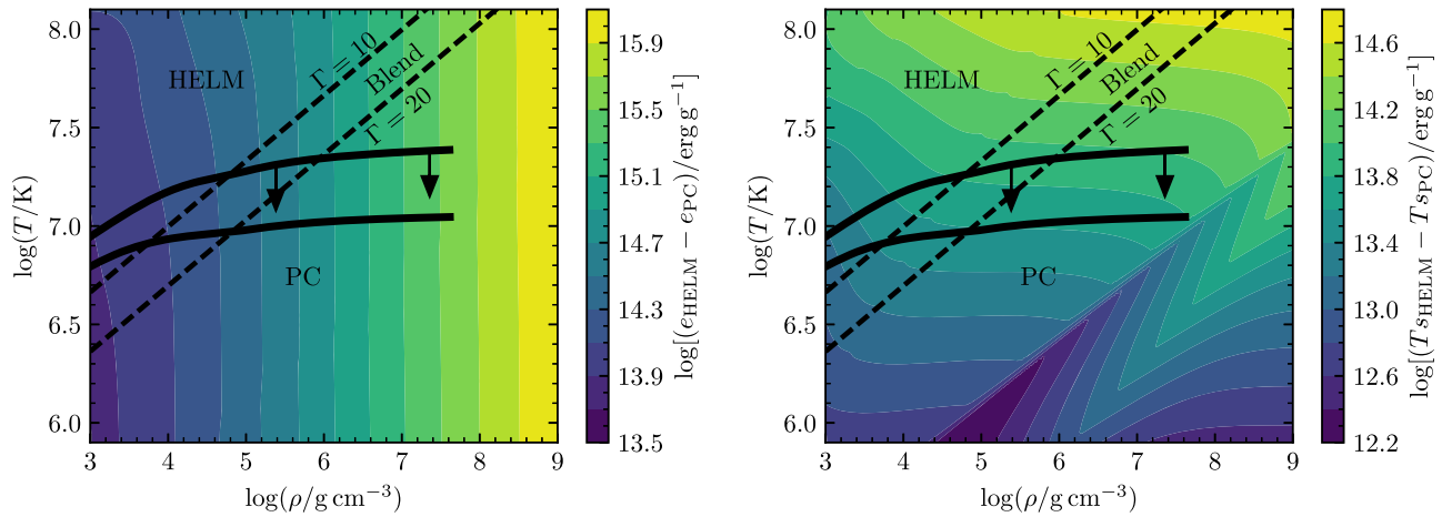
Figure 58. Magnitude of the energy differences between the HELM and PC EOS for specific internal energy e (left) and entropy s (right) in a 50/50 C/O mixture. Dashed lines show the EOS blending boundaries for 10 \leq \Gamma \leq 20 , and the solid black lines show representative profiles for a 1.0 M_{\odot} WD cooling from T_{\text{eff}} = 26,000 K to T_{\text{eff}} = 17,000 K.
