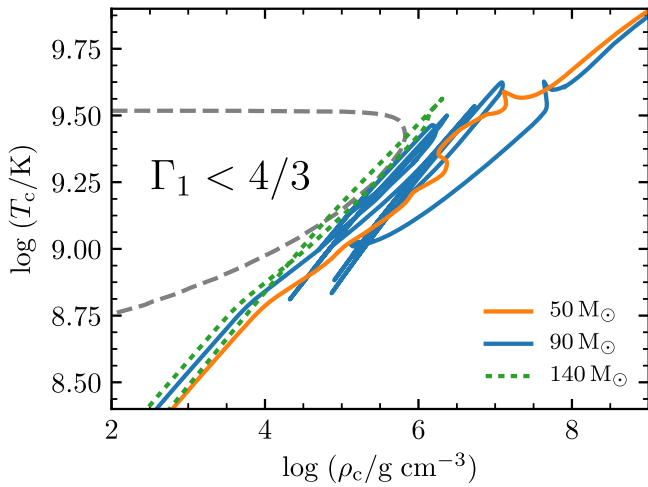
Figure 49. Central temperature and density for models with metallicity Z = 0.001 undergoing core collapse ( 50 M_{\odot} ), PPISN ( 90 M_{\odot} ), and PISN ( 140 M_{\odot} ).
