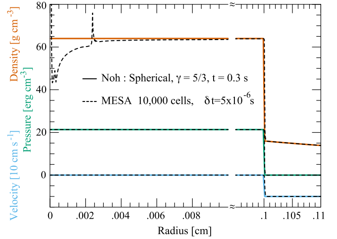
Figure 22. Analytic (colored solid) and MESA (black dashed) solutions for the density, pressure, and velocity at t = 0.3 \text{ s} in the Noh problem. Disagreements near the center are due to wall-heating, as discussed in the text.
