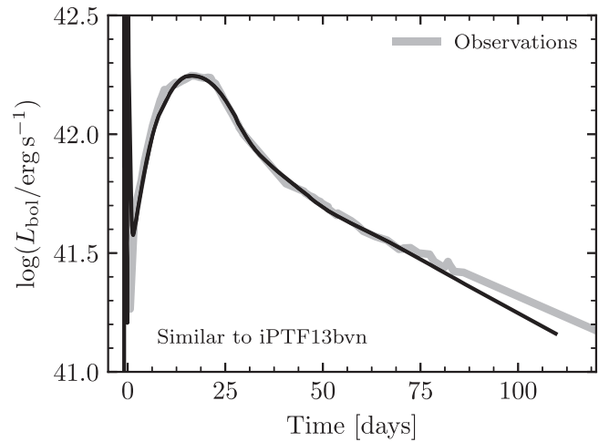
Figure 47. Comparison of a model (13bvn) similar to the stripped Type Ib SN iPTF13bvn with the observed bolometric light curve.
