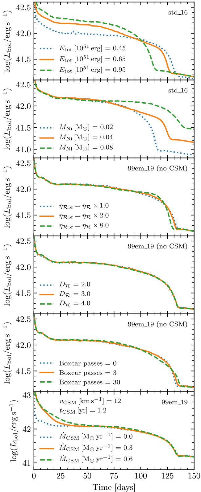
Figure 40. Effect of single-parameter variations associated with the SN explosion. Unvaried parameters have the values of the model listed in the upper-right corner of that panel.
