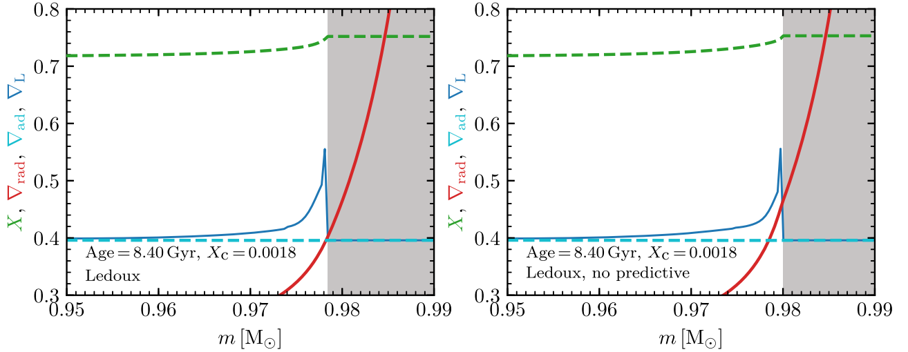
Figure 10. Profiles of \nabla_{\text{rad}} , \nabla_{\text{ad}} , \nabla_L , and X as a function of mass coordinate, in the outer envelope of the 1 M_{\odot} stellar model at an age of 8.40 Gyr. The panels show the separate runs described in the text. Gray shading indicates regions undergoing convection.
