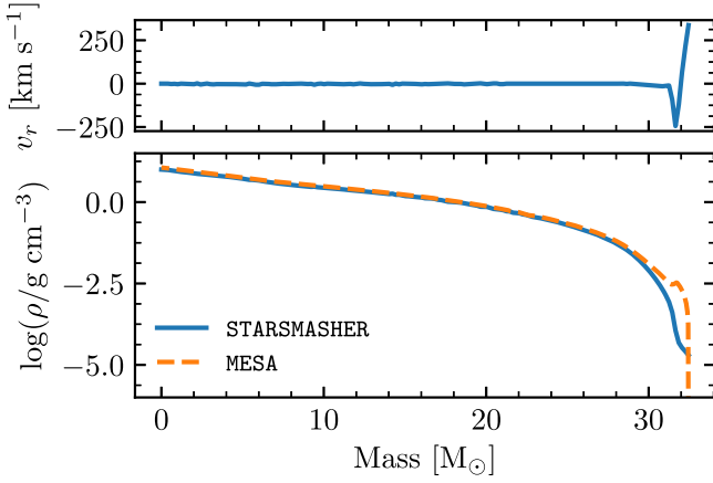
Figure 61. Mass-weighted spherical averages of radial velocity and density from the STARSMAHER simulation of a head-on collision between non-rotating 20 M_{\odot} and 15 M_{\odot} stars. The dashed line shows the resulting density profile of a MESA model relaxed to the entropy and composition profile of the simulation.
