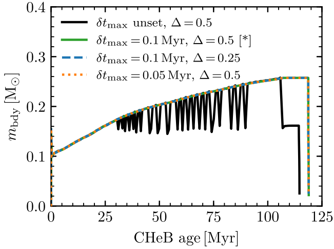
Figure 13. Mass coordinate m_{\text{bdy}} of the convective-core boundary plotted as a function of CHEB age, for the 1 M_{\odot} stellar model. Different line styles/colors show the separate runs with alternative time step ( \delta t_{\text{max}} ) and mesh resolution ( \Delta ) choices. The choices adopted in Section 2.4 are marked with an asterisk [*].
