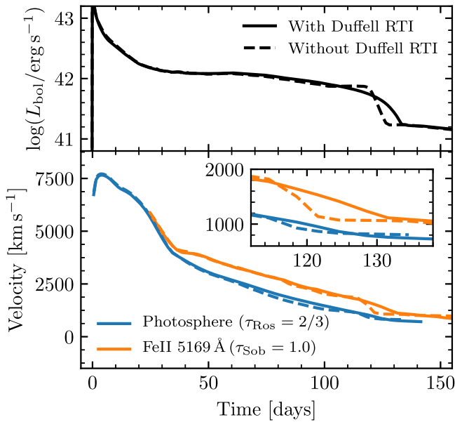
Figure 37. Effect of the Duffell RTI on the light curves (upper panel) and velocities (lower panel) of a Type IIP SN model (99em_19) similar to SN 1999em. The inset shows the time near day 120 where the altered density structure causes a significant difference in the Fe II line velocities.
