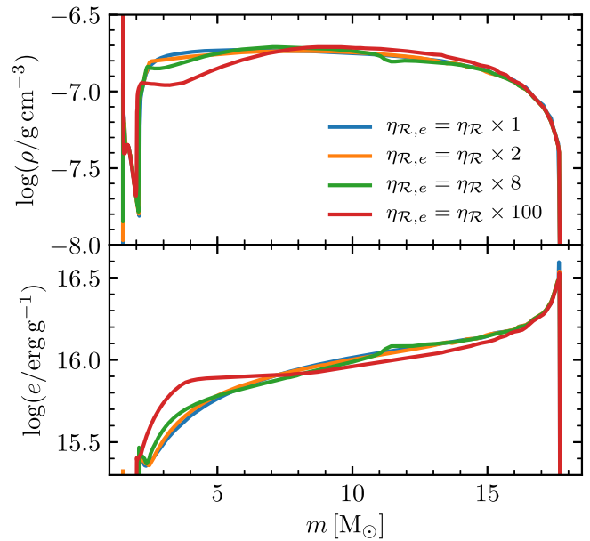
Figure 38. Structural effect of the RTI energy diffusion coefficient \eta_{\mathcal{R},e} . Other parameters are the same as in model 99em_19. The profiles are shown just before shock breakout. The effects on the light curve are shown in Figure 40.
