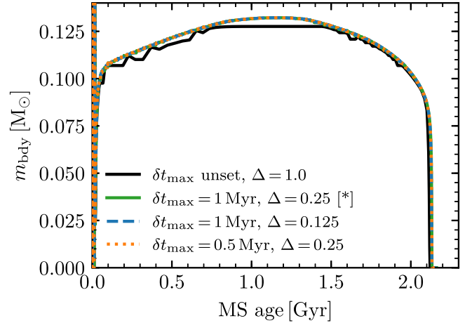
Figure 12. Mass coordinate m_{\text{bdy}} of the convective-core boundary plotted as a function of MS age, for the 1.5 M_{\odot} stellar model. Different line styles/colors show the separate runs with alternative time step ( \delta t_{\text{max}} ) and mesh resolution ( \Delta ) choices. The choices adopted in Section 2.2 are marked with an asterisk [*].
