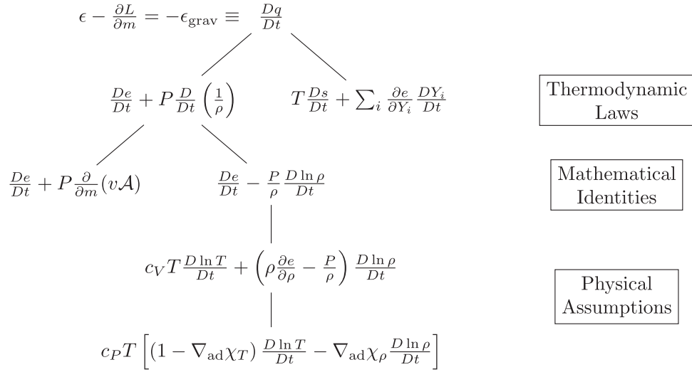
Figure 52. Schematic showing the relationships in Equations (59)–(65).
