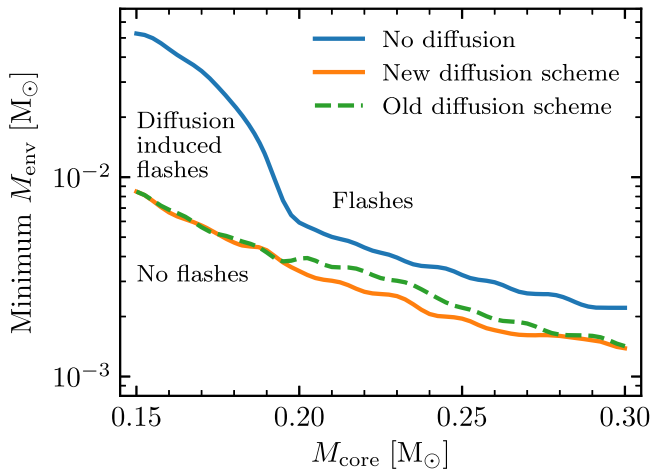
Figure 17. Minimum envelope mass M_{\text{env}} for which a H shell flash occurs on a He WD core mass M_{\text{core}} for Z = 0.02 MESA models with and without diffusion. The regime for the phenomenon of diffusion-induced flashes lies between the boundaries for models with and without diffusion.
