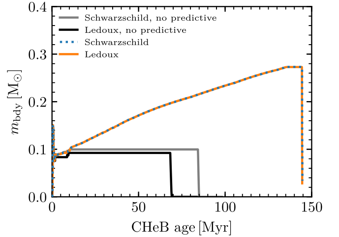
Figure 7. Mass coordinate m_{\text{bdy}} of the convective-core boundary plotted as a function of CHeB age, for the 3 M_{\odot} stellar model discussed in Section 2.4. Different line styles/colors show the separate runs described in the text.
