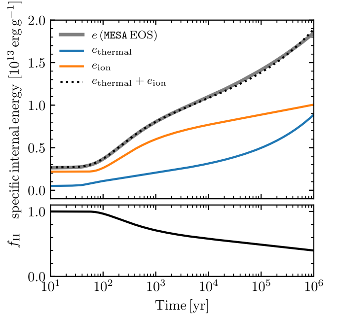
Figure 54. Specific internal energy at a fixed Lagrangian coordinate in the pre-MS model (upper panel). The solid colored curves indicate the individual energy terms. The internal energy reported by MESA (solid gray curve) exceeds the thermal energy because of the ionization energy. The lower panel shows the neutral fraction of the H.
