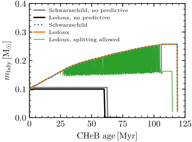
Figure 5. Mass coordinate m_{\text{bdy}} of the convective-core boundary plotted as a function of CHeB age, for the 1 M_\odot stellar model discussed in Section 2.4. Different line styles/colors show the separate runs described in the text.
