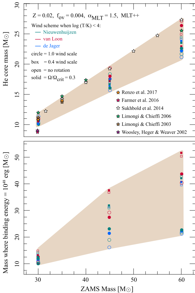
Figure 48. He core mass (upper panel) and mass location where the gravitational binding energy is equal to 10^{48} erg (lower panel) for ZAMS masses of 30, 45, and 60 M_{\odot} . Three stellar wind treatments, two wind scaling factors, and two rotation rates are shown for each ZAMS mass. The variation, illustrated by the tan band, induced by these modeling choices increases with ZAMS masses. Also shown are models from the literature (Woosley et al. 2002; Limongi & Chieffi 2003, 2006; Sukhbold & Woosley 2014; Farmer et al. 2016; Renzo et al. 2017), although each adopts different modeling choices and definitions of the He core mass.
