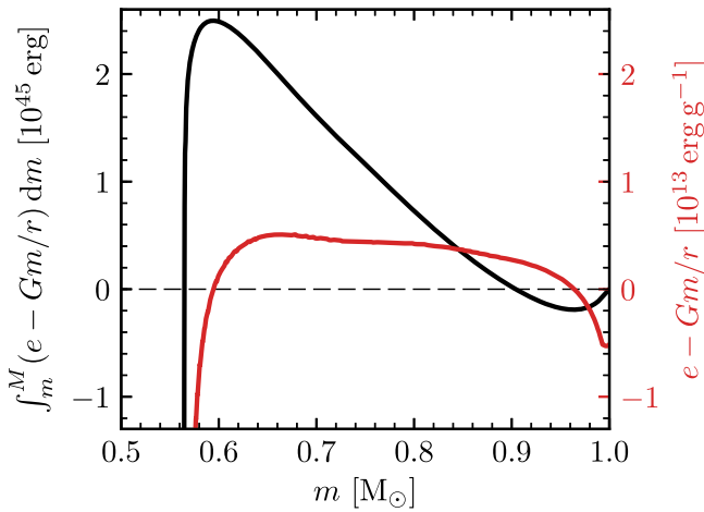
Figure 56. Specific (red) and cumulative (black) total energy (IE + PE) in the envelope of an AGB model ( M = 1.0 M_{\odot} , L = 4.97 \times 10^3 L_{\odot} , T_{\text{eff}} = 2,920 \text{ K} , R = 276 R_{\odot} ). This energy is positive in the envelope due to the inclusion of ionization energy in the internal energy reported by MESA.
