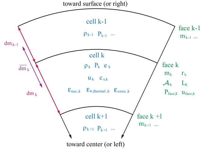
Figure 19. Cell and face variables relevant for hydrodynamics in MESA when using HLLC.
