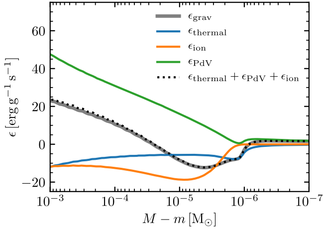
Figure 53. Value of \epsilon_{\text{grav}} in the pure-H pre-MS model, evaluated over a region near the stellar surface that includes an ionization zone (where \epsilon_{\text{ion}} \neq 0 ). The solid colored lines indicate the individual energy terms. Their sum (dotted black line) agrees with the value calculated by MESA (solid gray line).
