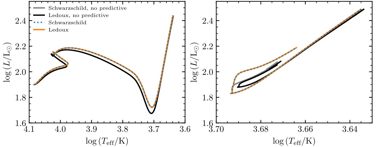
Figure 8. Evolution of the 3 M_{\odot} stellar model on the HR diagram, from ZAMS to the beginning of CHeB (left), and throughout the CHeB phase (right). Separate tracks show the different cases considered in the text; in the left panel, the Schwarzschild track without predictive mixing lies beneath the tracks with predictive mixing.
