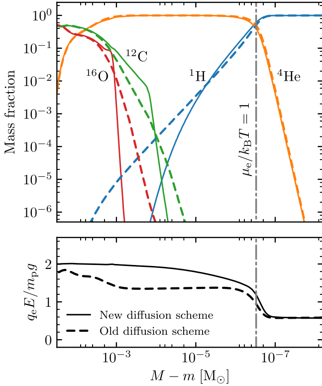
Figure 16. Abundance profiles in 0.6 M_{\odot} MESA WD models at T_{\text{eff}} = 5000 K after evolving for 4 Gyr to approach diffusive equilibrium in the outer layers. The old equations assume an ideal gas; the new equations include the effects of electron degeneracy.
