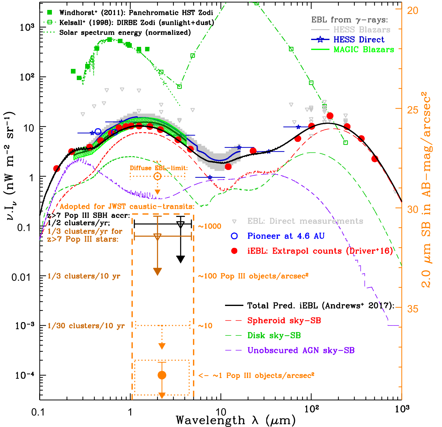
Figure 1. Summary of panchromatic backgrounds relevant to possible cluster caustic transits of Pop III stars and their stellar-mass black hole accretion disks. Green dotted-dashed lines with green unfilled squares indicate the scattered and thermal zodiacal foreground of Kelsall et al. (1998). Filled green squares indicate the panchromatic on-orbit zodiacal (labeled “Zodi”) foreground values measured by HST (Windhorst et al. 2011). Light gray unfilled triangles indicate direct measurements of the Extragalactic Background Light from low-Earth orbit or L2 (for a review, see Dwek & Krennrich 2013). Blue unfilled circles indicate the direct Pioneer spacecraft EBL values measured beyond most of the zodiacal dust at 4.6 au. Red filled circles indicate the integrated and extrapolated (to AB \gtrsim 30 mag) panchromatic galaxy counts (iEBL) of Driver et al. (2016 and references therein). The dashed red, green, and purple lines are iEBL model predictions for spheroids, disks, and unobscured AGNs, respectively (Andrews et al. 2017b). The solid black line is their total predicted iEBL. EBL constraints from H.E.S.S. \gamma -ray blazars are plotted as the light gray shaded region plus its dark-blue best fit, and for MAGIC blazars as the green shaded region with its dark-green best fit. The orange unfilled circle with dotted range is our “hard” upper limit for the diffuse 1–4 \mu m EBL, denoted as “Diffuse EBL-limit.” The orange dashed box contains our adopted upper limits on the 1–4 \mu m near-IR sky-SB for Pop III stars at z \gtrsim 7 (dark orange) and for their stellar-mass BH accretion disks at z \gtrsim 7 (black). The possible range in SB from Pop III objects is indicated at the level of \sim 1 , 10, 100, and 1000 objects/arcsec 2 . The filled orange circle indicates the approximate SB level of \sim 1 Pop III star/arcsec 2 . Cluster caustic transit rates that may be observed with JWST are listed in dark orange on the left for three SB levels, ranging from \sim 1 caustic transit per three clusters per year to \sim 1 per 30 clusters if monitored over 10 years. This is the lowest rate JWST could detect in a dedicated, large multiyear program. Details are given in Sections 2–7.
