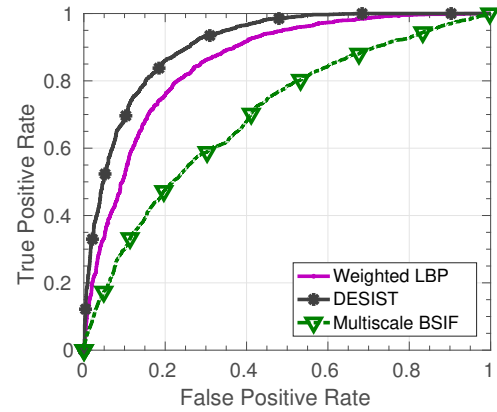
(a) Real vs Attack Iris Detection
