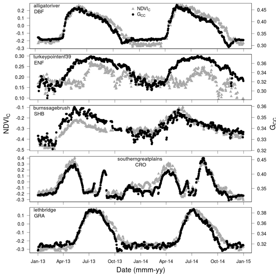
Fig. 1. Two-year of daily NDVI_C and G_{CC} from a selection of sites included in this study. DBF: deciduous broad-leaf forest; ENF: evergreen needle-leaf forest; SHB: shrubland; CRO: cropland; GRA: grassland.
