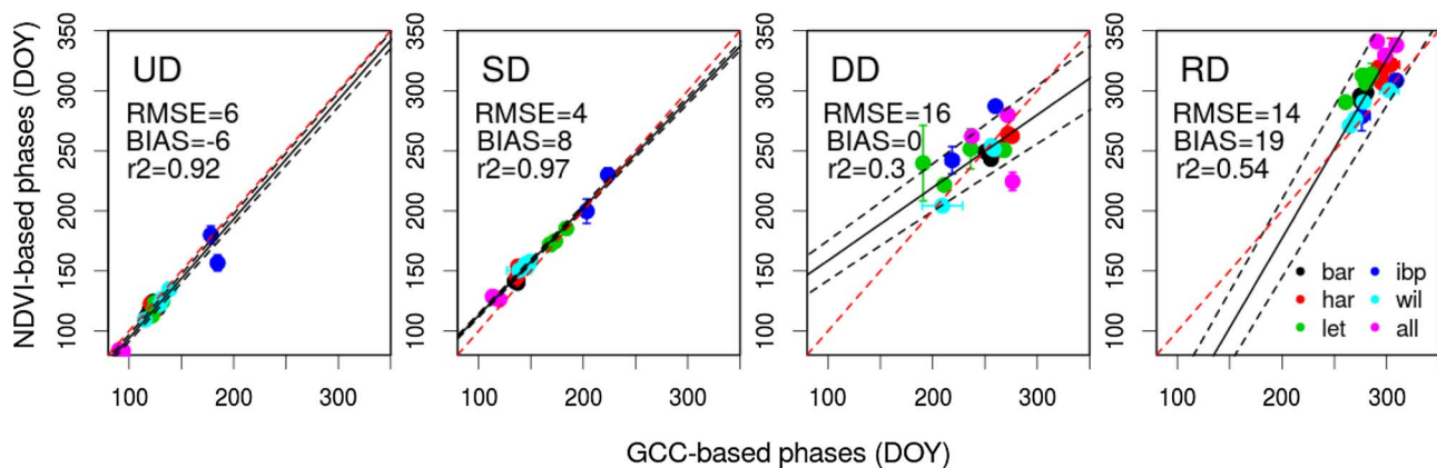
Fig. 2. Relationship between transition dates extracted from G_{CC} (x-axis) and NDVI_C (y-axis) time series for deciduous broad-leaf forests (DBF) and grasslands (GRA). Each data point is a site-year median date. Error bars represent the MAD. The red dashed line is the 1:1, whereas black lines represent the linear fit (solid) and its uncertainty (dashed). Site abbreviations: bar: bartlett; har: harvardbarn2; let: lethbridge; ibp: ibp; wil: willowcreek; all: alligatorriver. UD: upturn date; SD: stabilization date; DD: downturn date; RD: recession date. (For interpretation of the references to color in this figure legend, the reader is referred to the web version of this article.)
