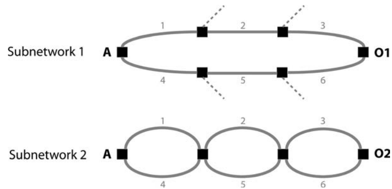
Figure A1. Illustration of two subnetworks with the same number of links but different topologic structure. Subnetwork 1: Apex connects to the outlet 1 (O1) via two paths, each composed of three links (note that the presence of vertices in the path implies for a delta system that other links (dashed lines) initiate at each of those vertices but drain to another outlet). Subnetwork 2: Apex drains to the outlet 2 (O2) via a more intricate structure.
