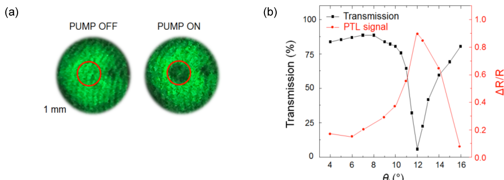
Fig. 2 Measurements of the PTL signal. a) Photographs of the reflected probe beam taken when the pump is switched off (left panel) and on (right panel). b) Transmission of the probe laser through the PC substrate and the PTL signals as a function of the incident angle.
