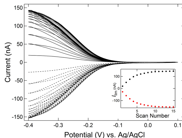
Figure 4. Repeated cyclic voltammograms of 1 \mu\text{M} \text{Ru}(\text{NH}_3)_6^{3+} scanned at the disk electrodes of an RRDE array, with ring electrodes at 0.1 V, in the absence of SE: ring current (solid) and disk current (dashed). (Inset) Variation of limiting current with the scan number: ring current (black) and disk current (red).
