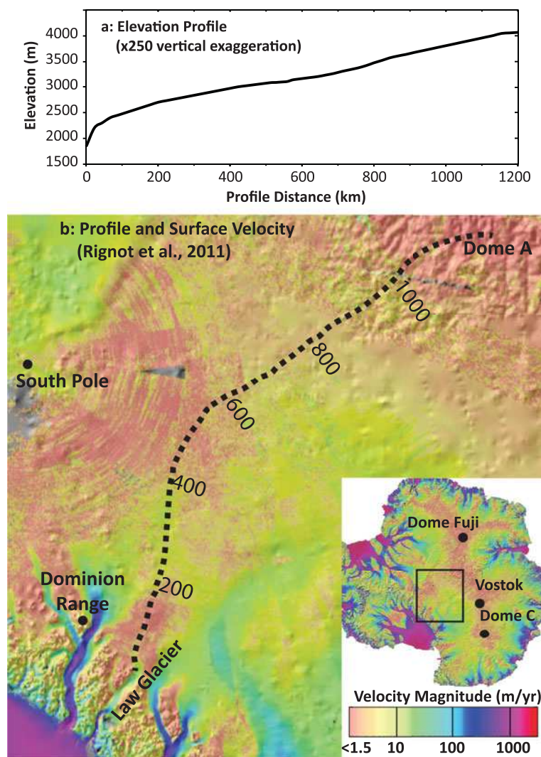
Fig. 7. Modeled flowline for ice supplied to Mount Acheron Moraine, based on MJ Hoffman's (personal communication) implementation of the Albany/FELIX model. The elevation profile for the flowline is shown in (a); modeled ice surface velocities from Rignot and others (2011) are shown in (b).
