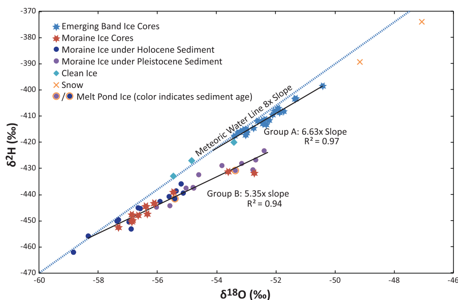
Fig. 4. Co-isotope plot depicting enrichment slopes from the global meteoric waterline. All analytical uncertainties are well within symbol size. Group A consists of the clean ice samples and samples from the Law Glacier ice cores. Group B consists of moraine ice samples and samples from the moraine ice cores. For group B in particular, the data are similar to results expected theoretically for regelation in an open system (Fig. 1). Also, local snow is isotopically enriched compared to any of the ice samples.
