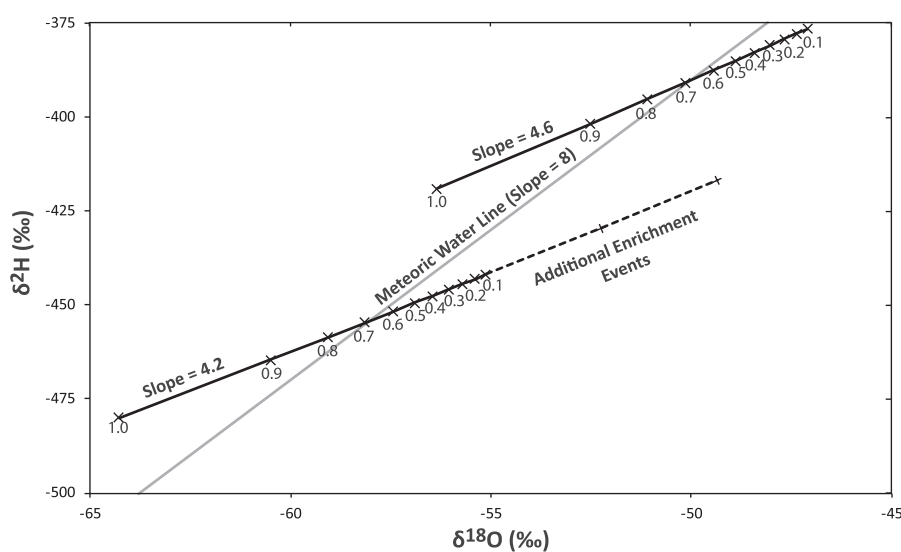
Fig. 1. Closed system theoretical freezing slopes (4.2 to 4.6) for initial meteoric water with initial two-isotope compositions of (−58‰, −454‰) and (−50‰, −390‰). Numbers reflect the fraction of the water that has frozen. The isotopic values of the remaining unfrozen water are plotted. Ice formed when \sim <2/3 of the water has frozen is enriched; the last \sim 1/3 of the refrozen ice is depleted. Thus, under open system refreezing where >1/3 of the melt is able to escape into the subglacial drainage, isotopic enrichment will be exclusively below the meteoric waterline. If the ice formed in a single refreezing event, enrichment of up to 2.9‰ \delta^{18}\text{O} is possible. The maximum effect of two subsequent open system melt and freeze enrichment events is illustrated for the lower freezing slope.
