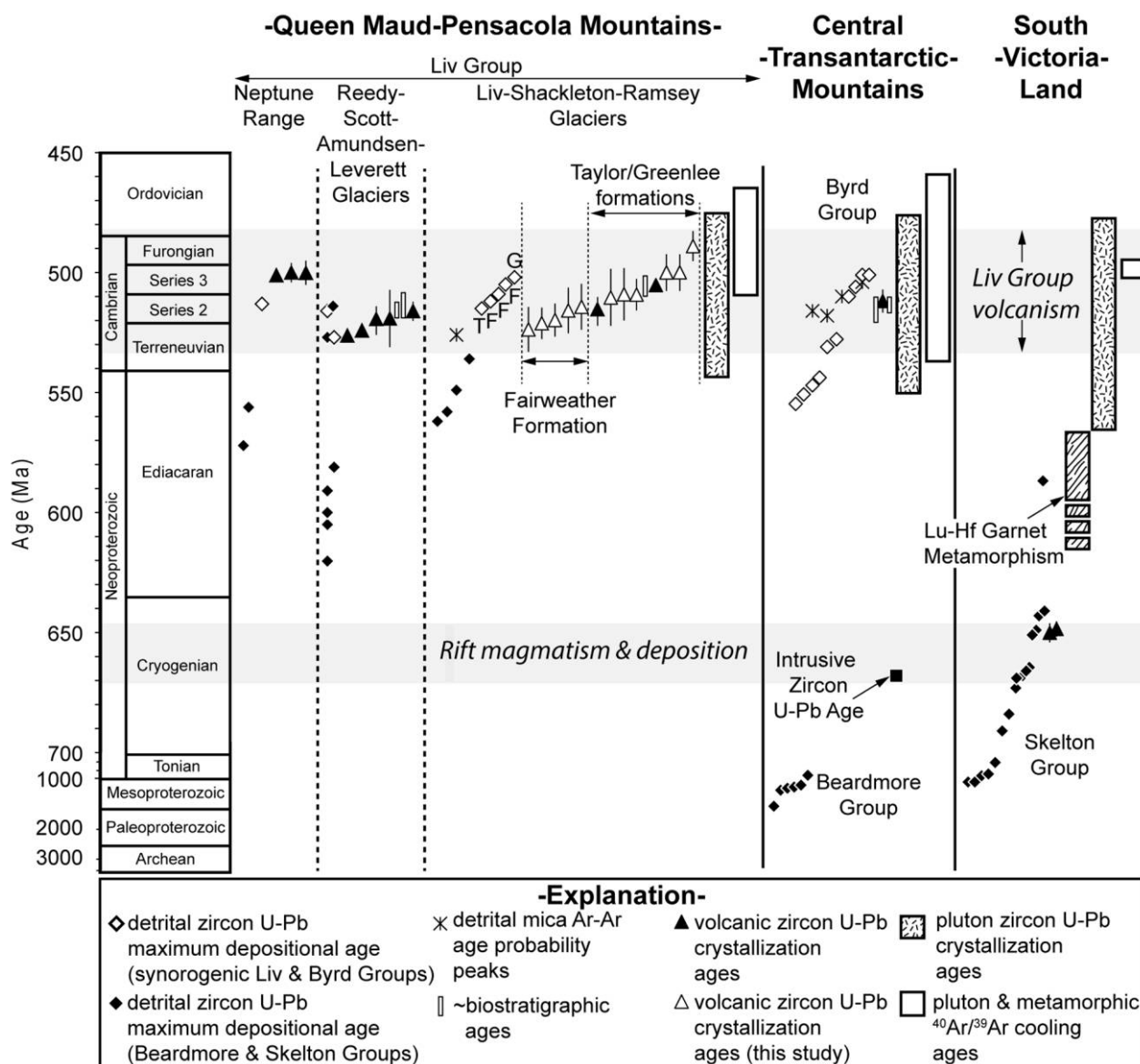
Figure 3. Diagram summarizing the available age constraints for the crystallization ages of volcanic and plutonic rocks, maximum depositional ages of siliciclastic rocks, and cooling ages of igneous and metamorphic rocks within the Queen Maud to Pensacola Mountains with respect to the central Transantarctic Mountains and south Victoria Land in the Ross orogen. Vertical black lines show errors on ages. Note the change in scale at 700 Ma. The Skelton Group in south Victoria Land includes the Koettlitz Group, following Gunn and Warren (1962) and Cook and Craw (2001). Ages are compiled from Goodge and Dallmeyer (1992, 1996), Rowell et al. (1992, 1993, 1997), Goodge et al. (1993, 2002, 2004a, 2004b, 2012), Hall et al. (1995), Millar and Storey (1995), Encarnación and Grunow (1996), Cooper et al. (1997), Van Schmus et al. (1997), Encarnación et al. (1999), Cox et al. (2000), Grunow and Encarnación (2000a, 2000b), Cook and Craw (2001), Allibone and Wysoczanski (2002), Mellish et al. (2002), Myrow et al. (2002), Read et al. (2002), Vogel et al. (2002), Curtis et al. (2004), Paulsen et al. (2004, 2008, 2013, 2015, 2017), Stump et al. (2004, 2006, 2007), Wysoczanski and Allibone (2004), Cottle and Cooper (2006a, 2006b), Talarico et al. (2007), Cooper et al. (2011), Hagen-Peter et al. (2015, 2016), and Martin et al. (2015). F = Fairweather Formation; G = Greenlee Formation; T = Taylor Formation.
