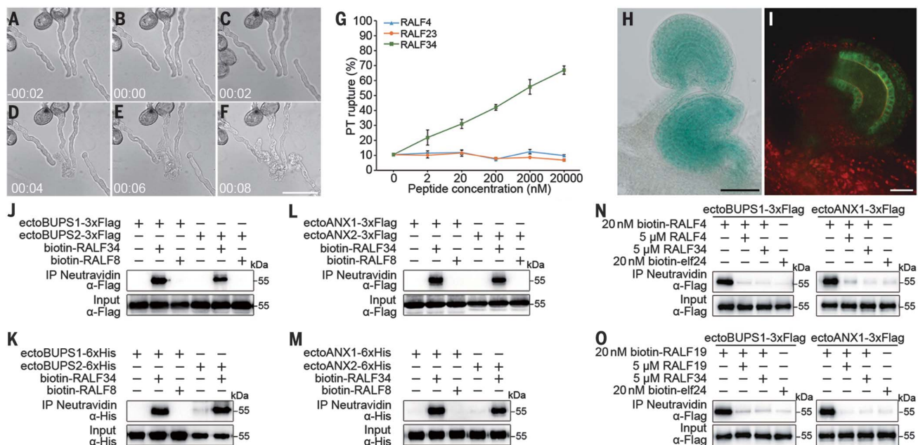
Fig. 4. RALF34 triggers pollen tube burst and interacts with and competes for the ANX-BUPS receptor complex. (A to F) Time-course imaging of pollen tube discharge induced by RALF34 treatment; 20 \mu\text{M} peptide was used to test the effect on growing wild-type pollen tubes. The pollen tube discharge occurs less than 10 s after RALF34 treatment. (G) Quantitative analysis of pollen tube rupture treated with different concentrations of RALF4, RALF23, and RALF34. Data are means \pm SD ( n = 230 pollen tubes of each treatment for two independent
