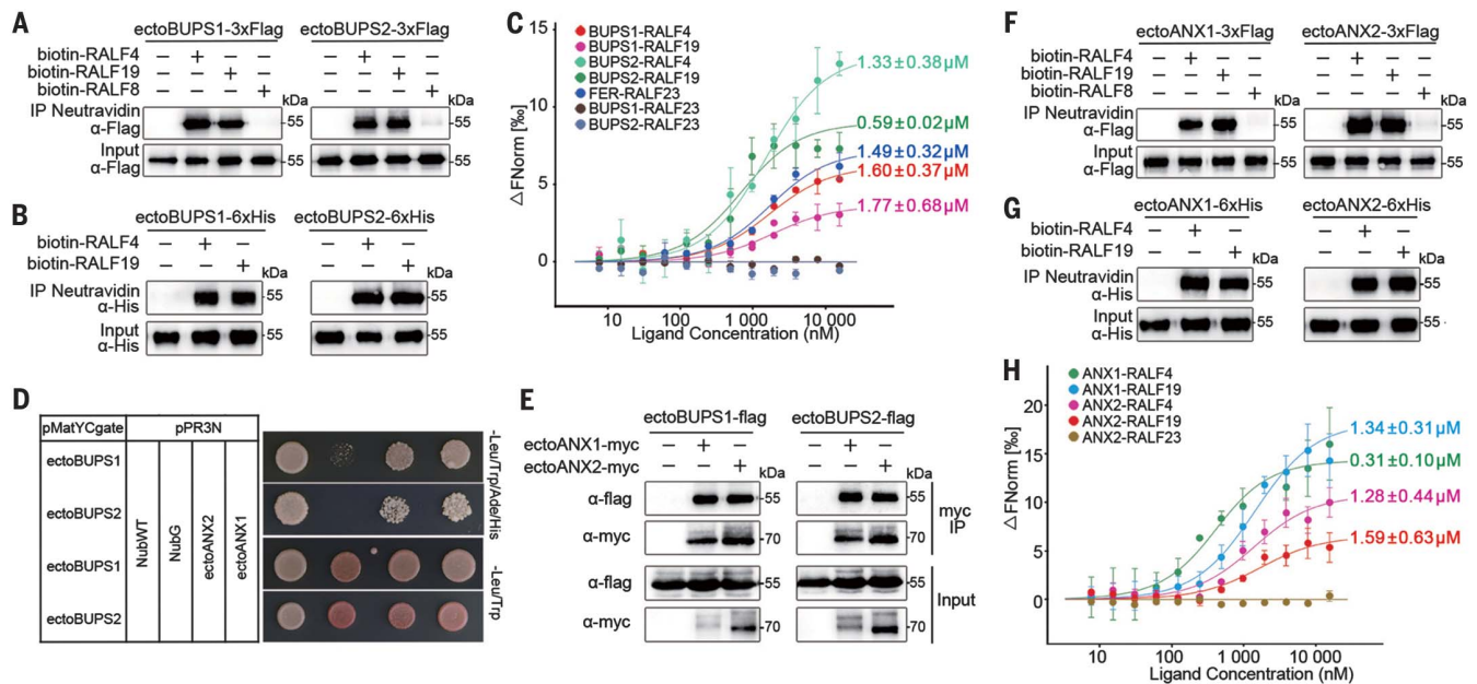
Fig. 3. BUPS1/2, ANX1/2, and RALF4/19 interact with each other. (A) Pull-down assay between Flag-tagged ectodomains of BUPS1/2 (purified from tobacco leaves) and biotinylated RALF4/19. (B) Pull-down assay between insect cell-expressed His-tagged ectodomains of BUPS1/2 and biotinylated RALF4/19. (C) Binding affinity between BUPS1/2 and RALF4/19 by MST analysis; K_d values are as indicated. The published RALF23-FER K_d value is 0.31 \mu\text{M} (24). \Delta\text{FNorm} , change in fluorescence. (D) Dual-membrane
