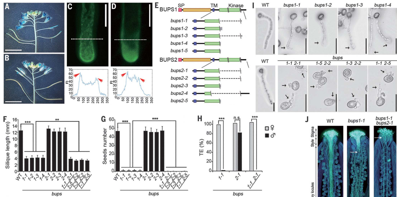
Fig. 1. Pollen-expressed BUPS1 and BUPS2 control pollen tube integrity. (A and B) Expression pattern of BUPS1 and BUPS2 , as shown by BUPS1p::GUS (A) and BUPS2p::GUS (B) in flowers. (C and D) Localization of BUPS1 -GFP (C) and BUPS2 -GFP (D) in pollen tubes. Graphs show fluorescence intensity (FI) 10 \mu m from the apex (denoted by white dashed line); the x-axis values represent the distance from the first dash at the left (in pixels) along the dashed line. Arrowheads indicate the fluorescence enrichment on the plasma membrane. (E) Mutant alleles of bups1 and bups2 . Double backslash (\\) denotes localization of single-guide RNAs; single backslash (\) denotes the mutation site; dashed lines indicate large chromosomal deletion. SP, signal peptide; TM, transmembrane domain. (F and G) Silique length (F) and number of seeds per silique (G) of the wild type (WT) and various mutants. Data are means \pm SD ( n = 20 siliques); *** P < 0.005 , **** P < 0.001 (Student t test). (H) Transmission efficiency of bups mutants. **** P < 0.001 ( \chi^2 test); n.s., not significant. (I) Pollen germination assay of bups1 and bups1 bups2 pollen grains. Pictures were collected after 7 hours of incubation. Arrows indicate the position of rupture. (J) Aniline Blue staining of WT, bups1 , and bups1 bups2 pollen tubes in wild-type pistils after 20 hours of pollination. Arrows show the areas where the bups pollen tubes made contact. Scale bars, 5 mm [(A), (B)], 10 \mu m [(C), (D)], 50 \mu m (I), 500 \mu m (J).
