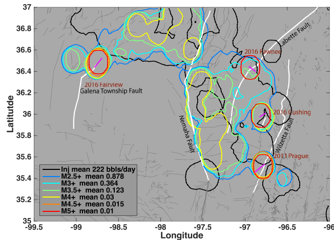
Figure 1. Map view of event density distribution for different sized earthquakes and injection rates. Colored lines show the contour lines of average distribution number of events for each magnitude range (see Legend). Gray lines show mapped faults from OGS database 86 . The major faults are labeled and shown in white thick lines. Thick purple lines denote the seismogenic faults for the four M5+ earthquakes delineated from earthquake locations. Each contour line represents spatial grids that have number of events larger than the average number of events per smoothed bin within the magnitude threshold. Individual density map is shown in Figure S1. The three M5+ sequences are well located at the edge of the seismic zones. The black contour line shows the spatial grids that have average injection rate from 2011 to 2016 higher than the average injection rate per smoothed bin. The figure is generated with Matlab 2015a, available at: http://www.mathworks.com/ .
