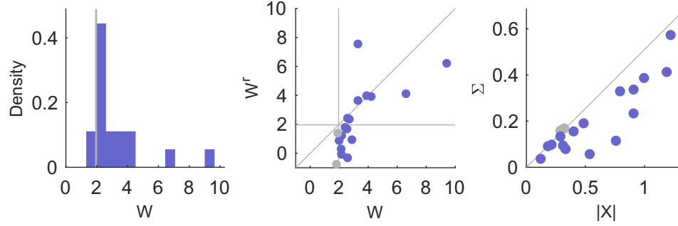
FIGURE 5. CAMERER ET AL. (2016) DATA
