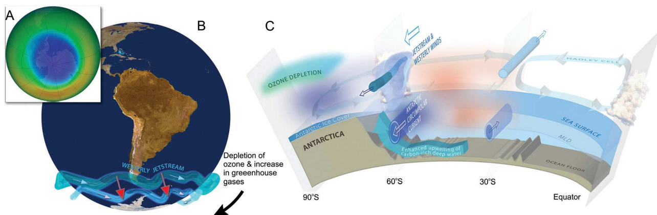
Fig. 6 The Antarctic ozone 'hole' (A) and its impact on Southern Hemisphere atmospheric and oceanic circulation. Stratospheric ozone depletion and resultant cooling over Antarctica have pulled the polar jet stream towards the South (B). The speed of the jet has also increased (see ref. 162 for details). The polar shift in the jet and its increased strength have changed atmospheric and oceanic circulation throughout the Southern Hemisphere (B). These changes are manifest in a mode of variability called the Southern Annular Mode (SAM). The atmosphere can be envisioned as balancing on a seesaw that is shifting up and down between the polar latitudes (south of 60°S) and a latitude band between 40–55°S. The seesaw moves up and down with changes in mean sea level pressure (MSLP). As it pivots, the large cells that drive the winds and precipitation move towards or away from Antarctica. When MSLP around Antarctica falls, the westerlies are strong, and SAM is in its positive mode; when MSLP rises over those same regions, the westerlies weaken, and SAM is in its negative mode. Over the past century, increasing greenhouse gases and depletion of ozone have pushed the SAM towards its more positive phase (black arrow in B). The main effects of the ozone 'hole'-induced positive phase of the SAM on the Southern Ocean are shown in C. The strengthening of the polar jet enhances the Antarctic Circumpolar Current and the associated overturning circulation (large blue-edged arrows). This drives increased upwelling of deep carbon-rich water and reduces the ability of the Southern Ocean to act as a sink for CO 2 . 164 South of the polar jet stream, temperatures have decreased (blue), while to the North, temperatures have increased (red). The mean SAM index is now at its highest level for at least 1000 years. 161 As a result, precipitation at high latitudes has increased and the mid-latitude dry-zone has moved south (see ref. 162 and 163). Clouds indicate areas with increased precipitation (over the equator and at the pole). (A. and B. were redrawn from ref. 165 and 162 with the ozone 'hole' over Antarctica in September 2017 reproduced from NASA Ozone Watch. 166 C. was reproduced from ref. 162).
