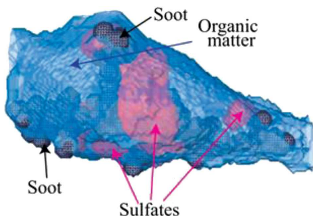
Fig. 12 An Aerosol particle collected in the atmosphere of Mexico City. Soot spherules, shown in black, are about 20 nm in diameter, and are emitted directly from combustion sources. The (false) colours show a coating of sulfate (red) and oxygenated organics (blue), produced by UV-initiated, \cdot\text{OH} -driven oxidation of sulphur dioxide and hydrocarbons (from ref. 435).
