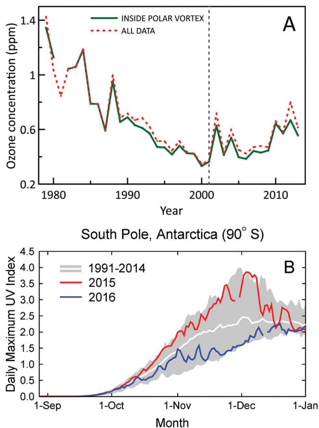
Fig. 1 (A) Time evolution of October, November, and December average concentrations of ozone in the lower stratosphere (about 10–20 km) over Antarctica derived from ozonesonde measurements at 11 stations (red-dashed line). Average concentrations derived from measurements inside the polar vortex are shown separately (green-solid line). Figure redrawn from ref. 2. (B) Daily maximum UV Index measured at the South Pole in 2015 (red line) and 2016 (blue line) compared with the average (white line) and the lowest and highest values (grey shading) of observations performed between 1990 and 2014. Measurements between mid-October and mid-December of 2015 and 2016 were, respectively, close to the upper and lower limits of historical observations. The figure is adapted from ref. 9 and updated with data from 2016.
