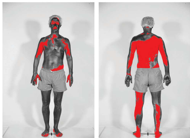
Fig. 5 The figure shows the skin coverage following application of sunscreen. Body areas covered in sunscreen appear dark, while the red colour shows skin surfaces not covered by sunscreen. The photographs were taken using standardised UV photography (UVP) that is sensitive only to the UV-A part of the spectrum. The sunscreen used absorbs incoming UV-A radiation. Therefore, body areas covered with these UV-A filters appear dark in UVP images. (Photograph from ref. 110 reproduced with permission).
