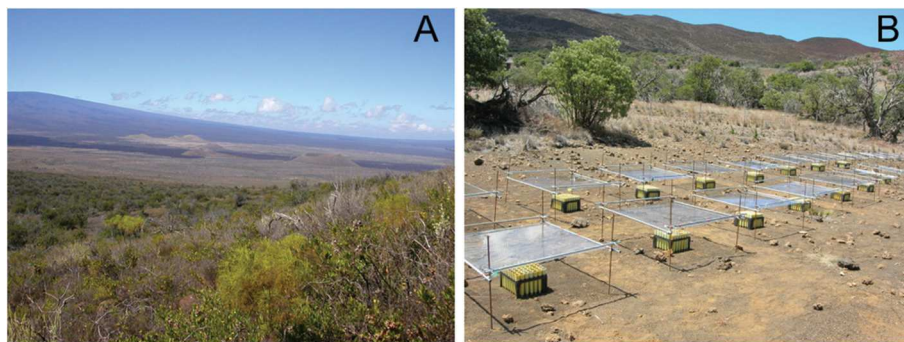
Fig. 7 Plants growing in high elevation tropical alpine locations, such as Mauna Kea, Hawaii (A), experience some of the highest natural levels of solar UV radiation at the Earth's surface. 213 These environments therefore provide excellent field sites for experiments designed to test the effects of extreme UV radiation conditions on plants (B). Shown here is an experiment using plastic film to reduce UV radiation to examine how these elevated levels of UV radiation influence plant growth and UV-screening. As plants migrate to higher elevations in response to climate change, they become exposed to higher levels of solar UV radiation as well as changes in several other abiotic and biotic factors. Understanding how plants will respond to UV radiation in the context of multiple environmental changes during migration is critical to assess how UV radiation and climate change will interact to modify the diversity and function of terrestrial ecosystems (Photographs by S. Flint).
