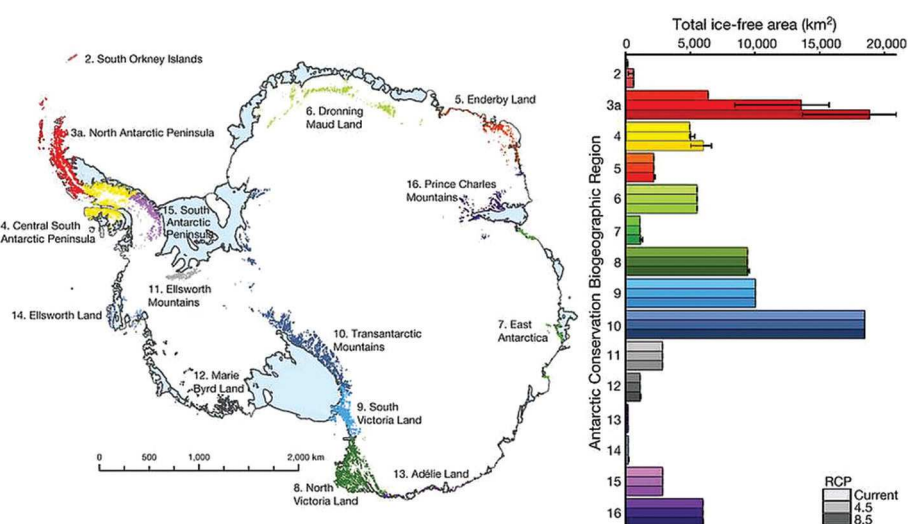
Fig. 10 Actual and projected future ice-free area in the Antarctic continent. New Antarctic ice-free area (km 2 ) predicted to emerge between 2014 and 2098 under climate forcing scenario RCP8.5 (Representative Concentration Pathway). Bar colours represent map locations of bioregions. Reprinted by permission from Macmillan Publishers Ltd.: J. R. Lee, B. Raymond, T. J. Bracegirdle, I. Chadès, R. A. Fuller, J. D. Shaw and A. Terauds, Nature , 2017, 547 , 49–54, ©2017 (ref. 377).
