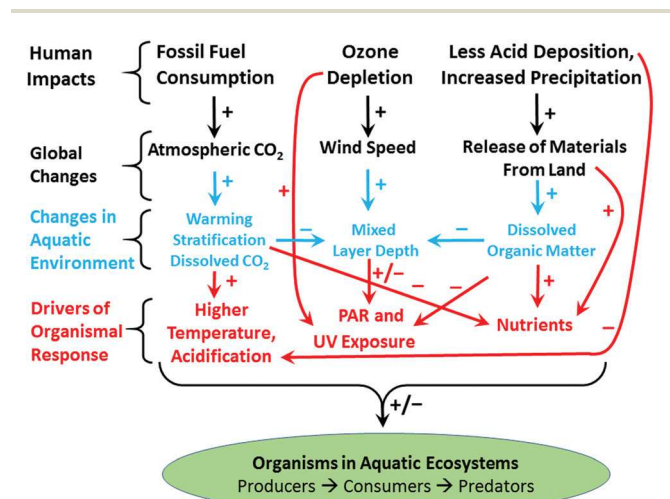
Fig. 8 Diagram to illustrate the processes by which various human activities affect exposure to UV radiation and other related aspects of the structure and function of marine and freshwater ecosystems. Anthropogenic drivers are leading to a suite of global changes, which in turn alter aquatic ecosystems and their primary producers, consumers, and higher-level predators. While marine systems are generally becoming more acidic due to anthropogenic CO 2 production, freshwater systems, on the other hand, are making extensive recoveries from previous anthropogenic acid deposition (acid rain) related to clean air act legislation in North America and Europe initiated in the early 1990s. However, this recovery from acidification is combining with increased precipitation to increase the concentrations of dissolved organic matter in some inland and coastal waters. Increased dissolved organic matter reduces the transparency of water to UV radiation (section 4.2), which, in turn, increases the survival of parasites and pathogens of humans and wildlife. 320
