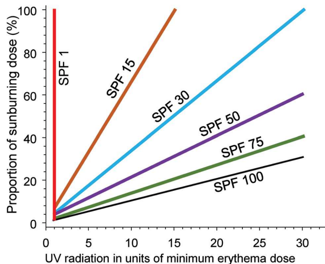
Fig. 4 The graph shows the effectiveness of sunscreen of different sun protection factors (SPF) for preventing sunburn. The dose of UV radiation (x-axis) is presented in units of the dose that will cause minimal erythema (MED) of the skin. The y-axis is the percentage of a sunburning dose (1 MED) that will be received by the skin, using sunscreens of different SPF. With no sunscreen (SPF = 1) a dose of UV radiation of 1 MED results in 100% of the dose required to cause sunburn. With successively higher SPF sunscreens, the dose of UV radiation required to reach 1 MED (100% of a sunburning dose) increases. Adapted from ref. 106.
