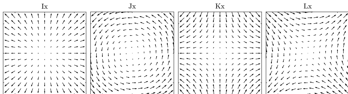
Figure 1. Matrix products associated with the IJKL matrices presented as quiver plots. From left to right, plots of Ix , Jx , Kx , and Lx are shown. These are the same as a velocity field of pure divergence, pure vorticity, pure normal strain and pure shear strain, respectively.
