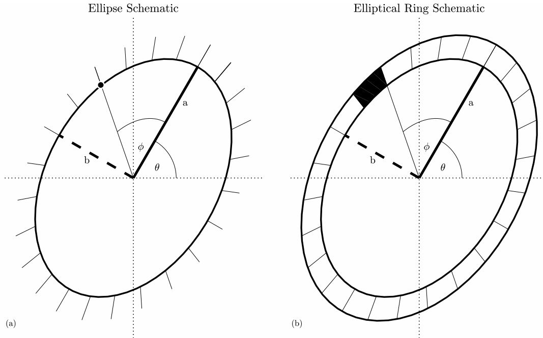
Figure 3. Schematics for (a) an ellipse and (b) an elliptical ring or annulus. In both panels, the semi-major and semi-minor axes a and b are denoted by heavy solid and heavy dashed lines, respectively, while the location of one particular particle along the periphery is marked with a thin solid line. The ellipse orientation angle \theta , measured counterclockwise from the x -axis, and the phase angle \phi to the particle location from the major axis are also shown. The ellipse marks uniform increments of \Delta\phi = \pi/48 radians in the phase angle \phi . In (b), two concentric ellipses of identical shape and orientation, but slightly different sizes, are drawn. The space between these two ellipses forms an elliptical ring or annulus , with the phase angle \phi now taken to mark parcels , shown later to have the same area, as opposed to simply a location around the ellipse periphery. The parcel between the indicated phase angle \phi and \phi + \Delta\phi is filled in with dark shading.
