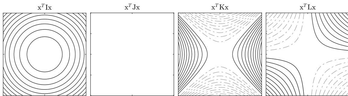
Figure 2. Quadratic forms associated with the \mathbf{IJKL} matrices. From left to right, contour plots of \mathbf{x}^T \mathbf{I} \mathbf{x} , \mathbf{x}^T \mathbf{J} \mathbf{x} , \mathbf{x}^T \mathbf{K} \mathbf{x} , and \mathbf{x}^T \mathbf{L} \mathbf{x} are shown, with positive contours shown as black solid lines and negative contours as dashed-dotted gray lines. Note that \mathbf{x}^T \mathbf{J} \mathbf{x} = 0 identically.
