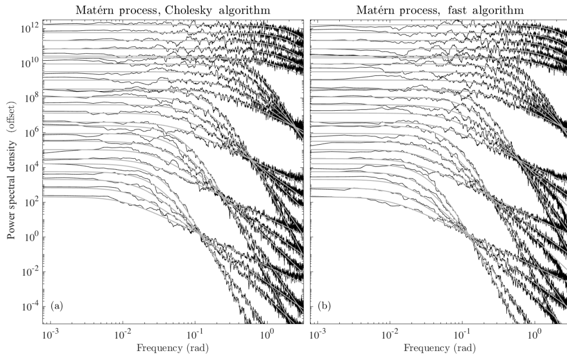
Figure 8. A comparison of the spectra of simulated unit-variance Matérn processes having 25 different (\alpha, \lambda) values for (a) the Cholesky decomposition algorithm and (b) the fast generation algorithm presented here based on the Green's function. The process samples are each 8000 points long, with the sample interval \Delta set to unity. Black curves show the multitaper spectral estimates, as described in the text, while gray curves are the theoretical spectral forms. Successive spectral plots have been offset in the vertical by a factor of \sqrt{10} for presentational clarity. The five lines within each group correspond to the five \alpha values 1, 1.5, 2, 3, and 4. The five groups correspond to different values of \lambda , with \lambda equal to 0.01, 0.02, 0.05, 0.2, or 1 times the value of \alpha for each curve, proceeding from bottom to top. Only positive frequencies are shown, as the theoretical spectra at negative frequencies are identical. Simulated spectra from the O(N \log N) fast algorithm in (b) and those from the O(N^3) Cholesky algorithm (a) are found to be virtually identical.
