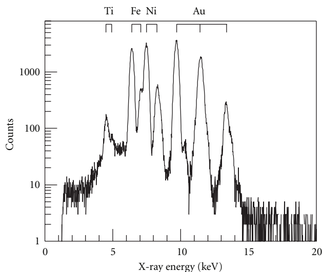
FIGURE 1: A PIXE spectrum of a NiFe thin film deposited from a 100 mM \text{NiSO}_4 , 10 mM \text{FeSO}_4 , 0.5 M \text{H}_3\text{BO}_3 , and 1 M \text{Na}_2\text{SO}_4 solution at -900 mV for 6 min. Approximately 1.8 \mu\text{C} of 3.4 MeV protons were incident on the sample to obtain this spectrum. The peaks corresponding to the K X-rays of Ti, Fe, and Ni, and the L X-rays of Au are indicated.
