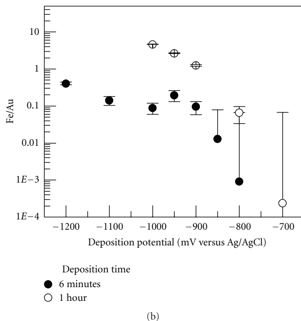
FIGURE 4: The (a) Ni/Au ratio and (b) Fe/Au ratio determined by PIXE as a function of the deposition potential for two different deposition times.
