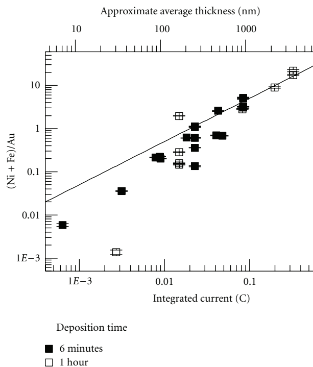
FIGURE 2: The (\text{Ni} + \text{Fe})/\text{Au} ratio determined by PIXE as a function of the integrated deposition current for all the samples. The deposition potentials varied from -700 mV to -1200 mV and the deposition times were either 6 or 60 min. The upper horizontal axis indicates an approximate average deposit thickness, calculated assuming 100% current efficiency. The solid line with a slope of unity is a guide to the eye. The (\text{Ni} + \text{Fe})/\text{Au} results fall below this line at lower integrated currents.
