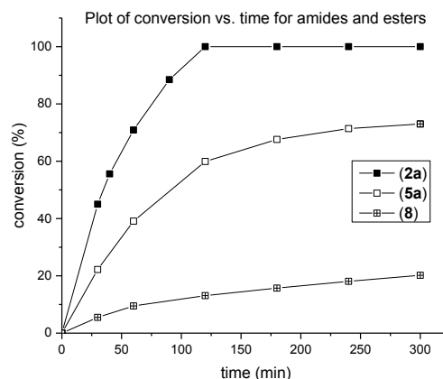
Figure 2 Kinetic profile in the Suzuki-Miyaura cross-coupling with 4-tolylboronic acid catalyzed by (1) (3 mol%) at room temperature. 2a : N,N -Ph,Boc; 5a : OPh; 8 : N,N -Ph,Ts.
