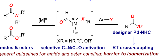
B: This work: the first room temperature coupling of amides and esters
