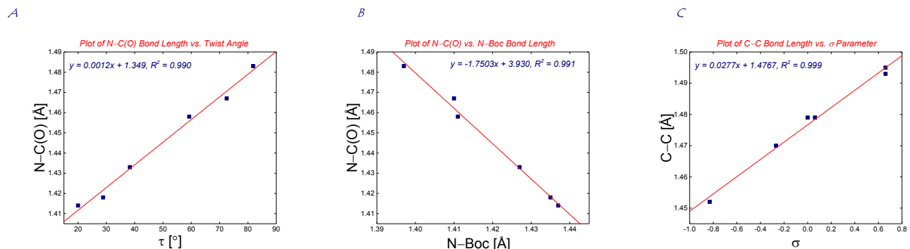
Chart 1. (a) Correlation of N-C(O) bond length [Å] to twist angle ( \tau ) for amides 2a-e . (b) Correlation of N-C(O) bond length [Å] to N-Boc bond length [Å] for amides 2a-e . (c) Correlation of C-C bond length [Å] to Hammett \sigma parameter for amides 2a-e (X-ray data).
