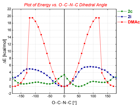
Figure 4. Correlation of \Delta E [kcal/mol] to O-C-N-C [°] in 2c , 2i and DMAc (N,N-Dimethylacetamide).
