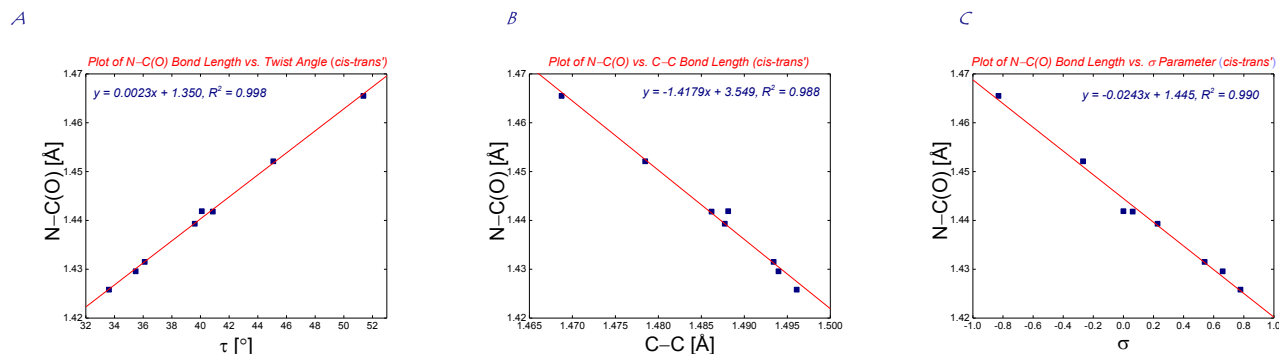
Chart 2. (a) Correlation of N-C(O) bond length [Å] to twist angle ( \tau ) for amides 2a-h . (b) Correlation of N-C(O) bond length [Å] to C-C bond length [Å] for amides 2a-h . (c) Correlation of N-C(O) bond length [Å] to Hammett \sigma parameter for amides 2a-h (cis-trans', B 3 LYP/6-311++G(d,p) data).
