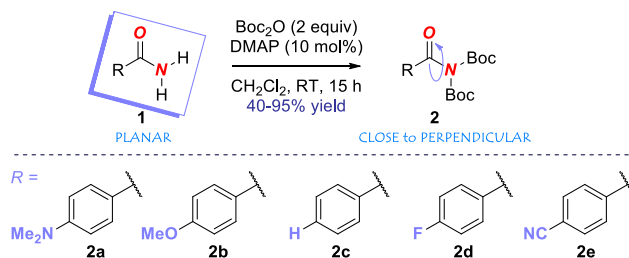
Figure 2. One-step synthesis of twisted amides.
