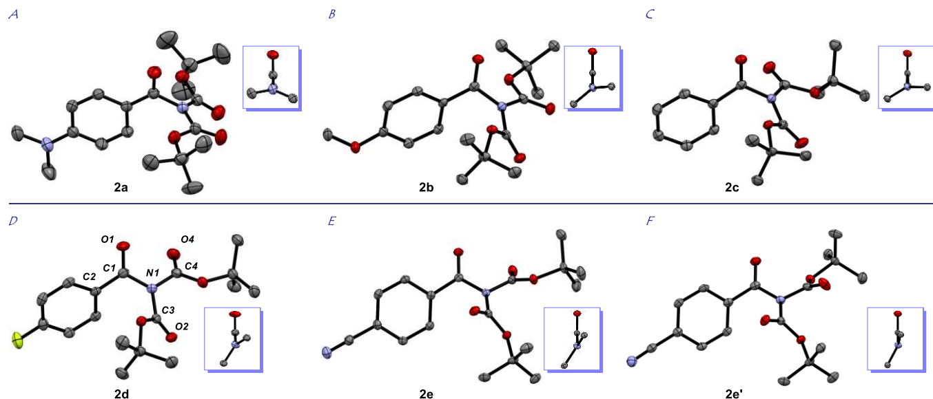
Figure 3. Crystal structures of amides 2a-e . 2e : two molecules in the unit cell. Insets show Newman projections along N–C(O) bonds.
