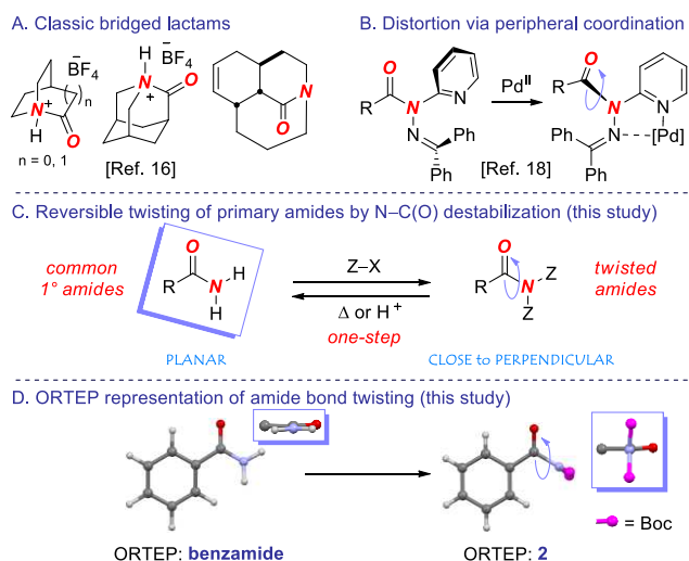
Figure 1. (a) Examples of highly distorted amides in cyclic frameworks (classic bridged lactams). (b) Amide distortion by peripheral coordination (Shibasaki et al.). (c-d) Reversible twisting of acyclic primary amides by ground-state N–C(O) destabilization (this study, insets show view along N–C(O) axis).
