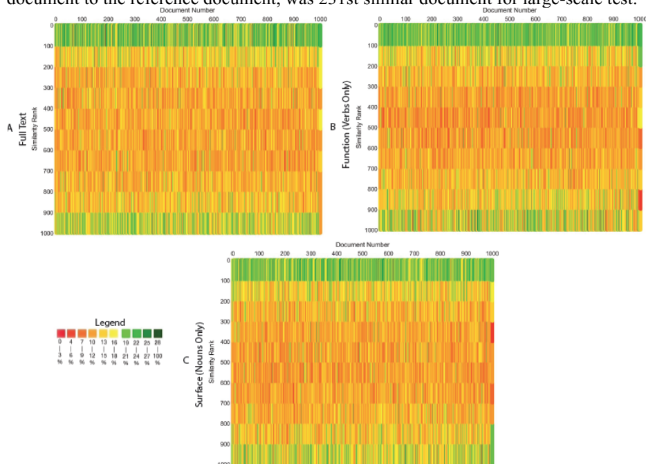
Fig. 4 Large-Scale Test Case with 1,000 Patents A) Using full text of patents, B) Using Only Functional Content of Patents (Verbs), C) Using Only Surface Content of Patents (Nouns)
