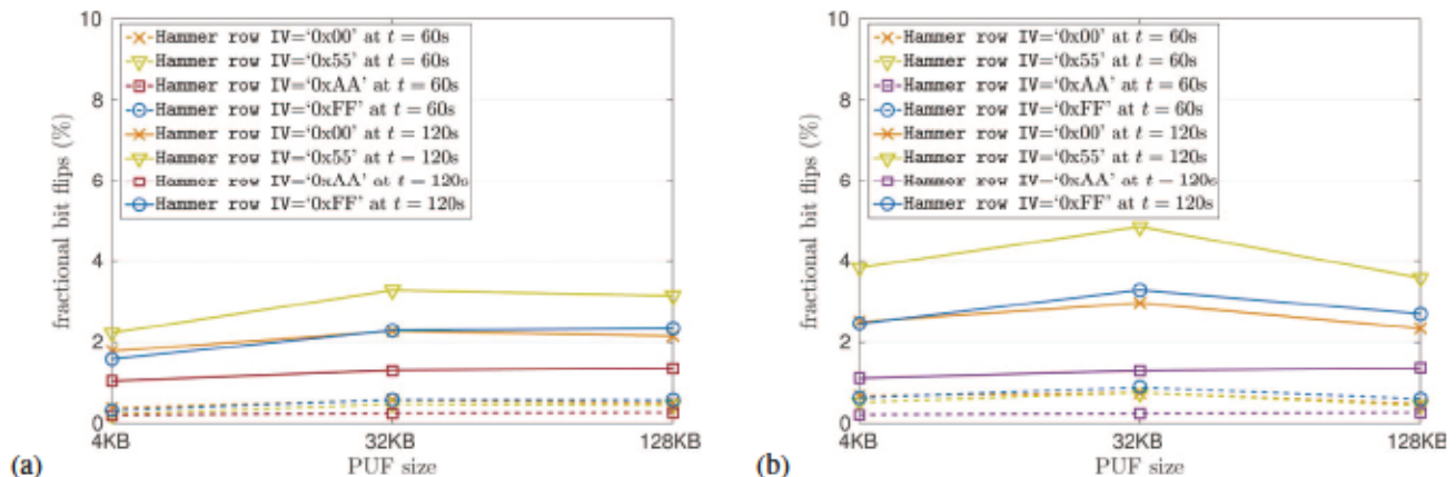
Fig. 3. Fractional number of bit flips, given in percent relative to PUF size, using PUF row IV='0xAA'. Left: number of bit flips using SSRH. Right: number of bit flips using DSRH.
