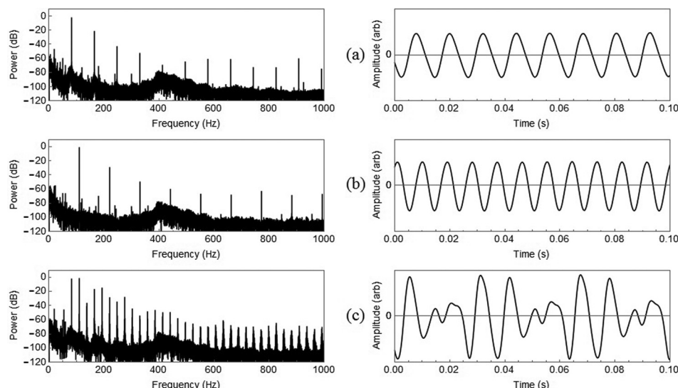
Fig. 4. Power spectra and waveforms of the sound produced by the piano when driven by (a) the shaker oscillating at frequency f_3 only, (b) the shaker oscillating at frequency f_4 only, and (c) both shakers oscillating simultaneously. In each case the shakers were oscillating at the maximum available amplitude. All strings were damped.
