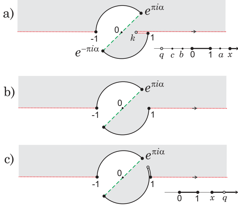
Figure 10: A global family of special pentagons
