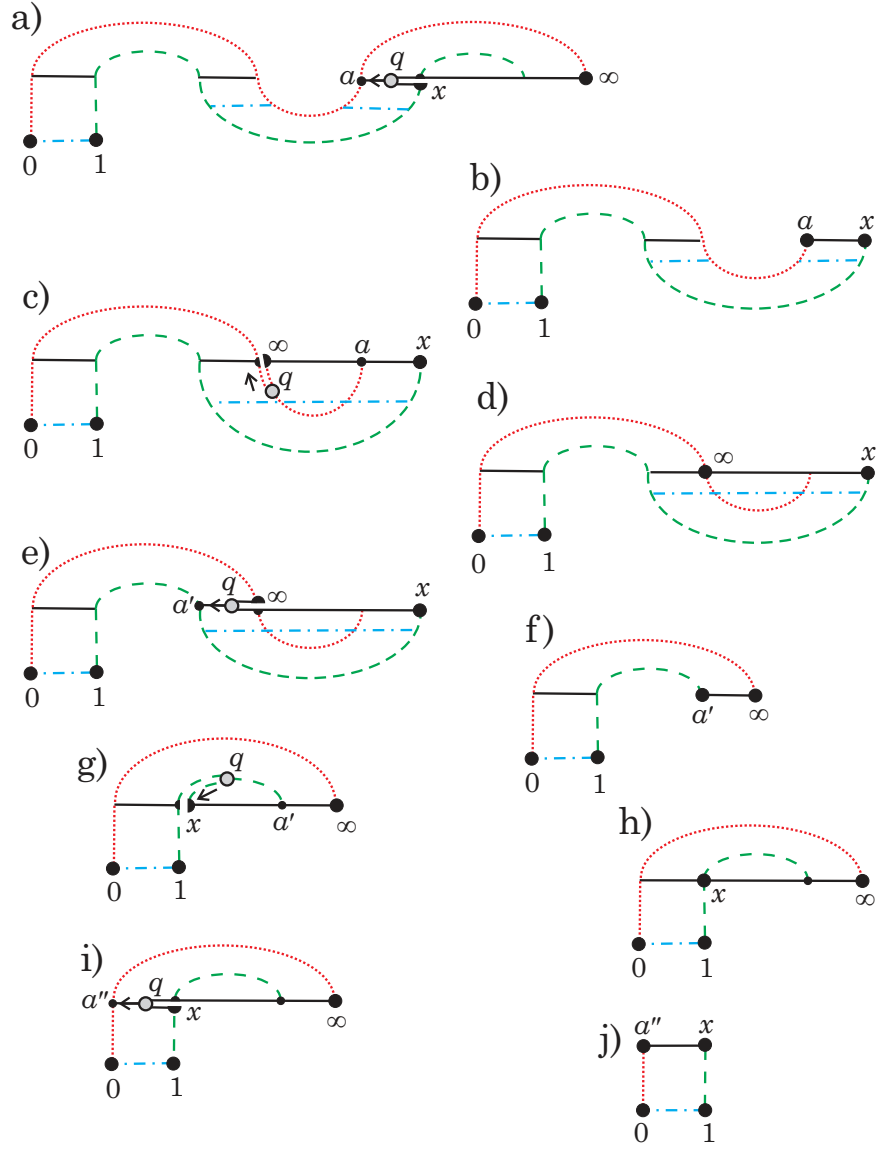
Figure 22: Nets for a part of the global family in Example 6.
