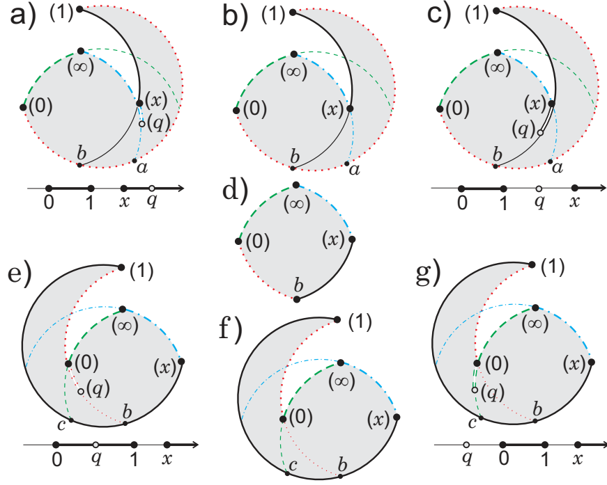
Figure 13: Global family in Example 2.
