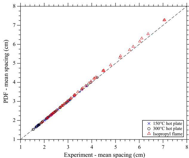
Fig. 9. Displayed here are comparisons of the mean streak spacings from the experimental data vs. the means of the fitted lognormal distribution. Data is taken from both tested hot plate temperatures as well as the isopropyl fuel wick. The dashed line indicates the line of unity.
