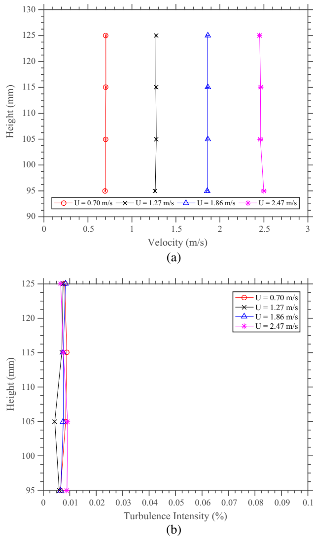
Fig. 4. (a) Plot of freestream velocity values at several heights in the center of the wind tunnel. Horizontal error bars indicate one standard deviation. (b) Plot of the turbulence intensity levels in the freestream flow at the center of the wind tunnel.
