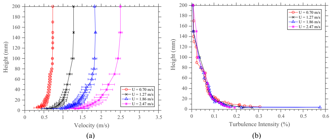
Fig. 5. (a) Height vs. velocity measured 1.5 cm upstream of the hot plate leading edge. Horizontal error bars indicate one standard deviation of the velocity data. (b) Height vs. turbulence intensities measured 1.5 cm upstream of the hot plate leading edge.
