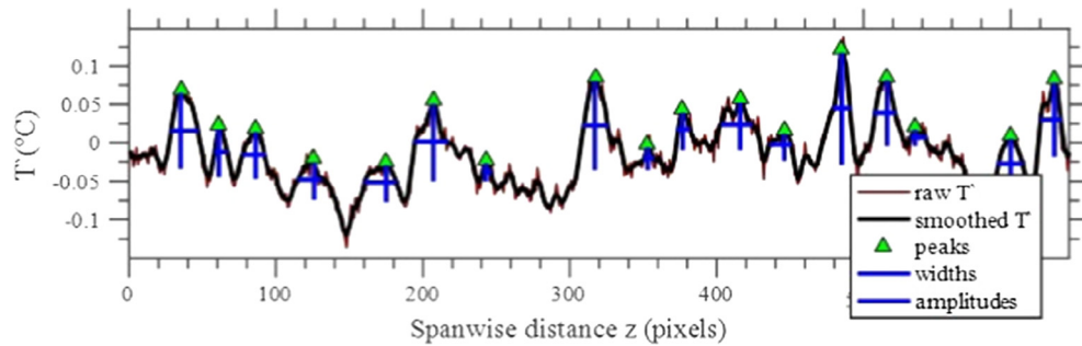
Fig. 21. Example of the streak detection algorithm with displayed results for one image. Here, the raw T' profile is shown as a thin red line while the smoothed profile is shown as the thicker black line. This image also shows derived streak locations or peaks (green triangles), streak widths (horizontal blue lines), and streak amplitudes (vertical blue lines). (For interpretation of the references to color in this figure legend, the reader is referred to the web version of this article.)
