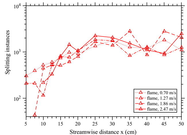
Fig. 20. A semilogarithmic plot of the instances of streak splitting observed in a 5 s period. The isopropyl fuel wick is located between x = 0 and x = 20.5 cm.
