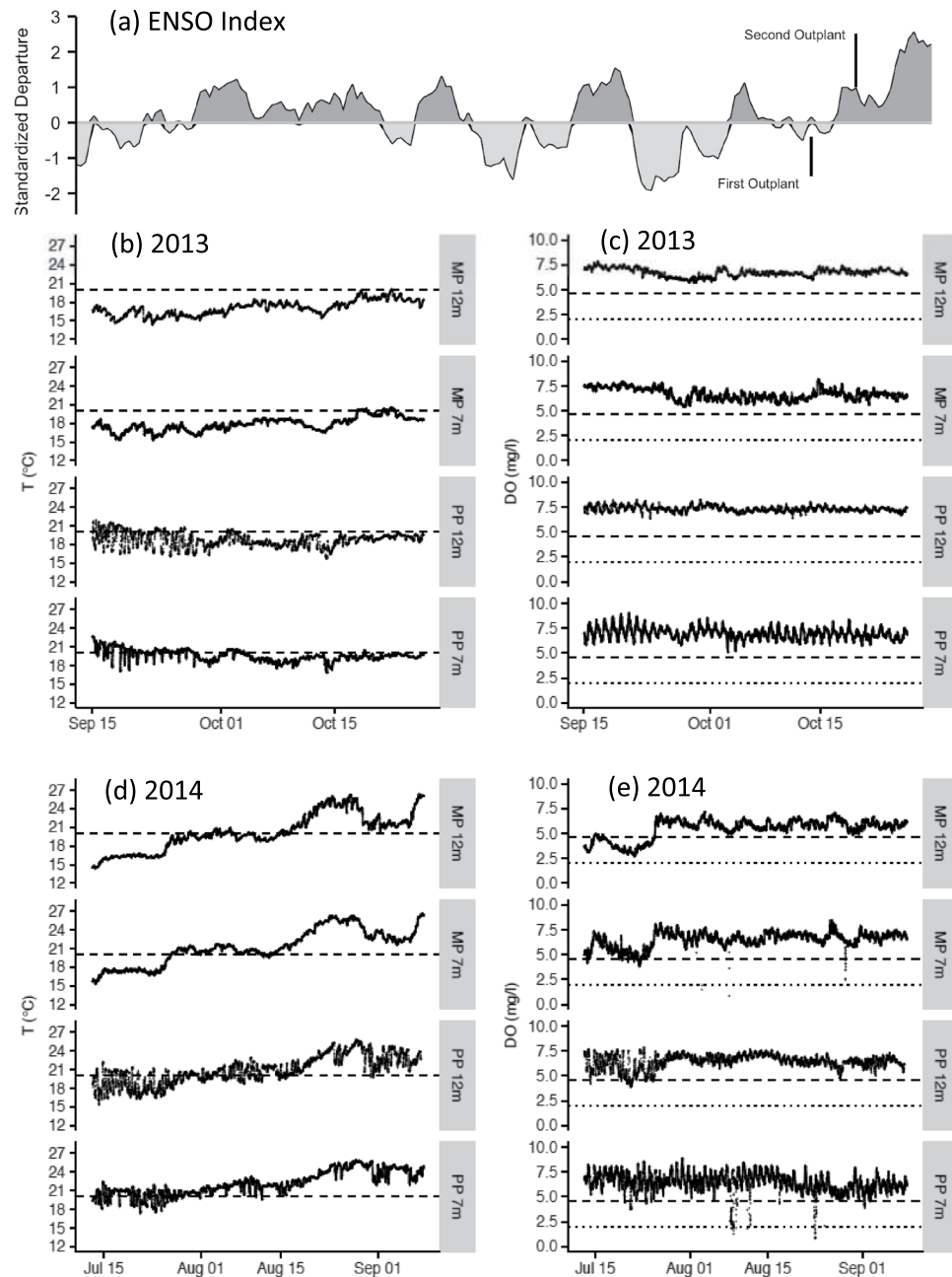
Figure 2. Climate and local oceanographic conditions during the in situ abalone experiments. (a) Recent NOAA estimates of ENSO oscillations (from https://www.esrl.noaa.gov/psd/enso/mei/table.html ). Initial times for both abalone outplants are indicated on the index. (b,d) Sep. – Oct. 2013 and July – Sep 2014 time series of seawater temperature (°C) at the 4 abalone outplant locations. Dashed black lines represent the 20 °C temperature reference used to derive the Temperature Index (TI). (c,e) Sep – Oct 2013 and July – Sep 2014 time series of dissolved oxygen concentration (mg/l) at the 4 outplant locations. Long dashed black lines represent the sub-lethal levels of dissolved oxygen (4.6 mg/l) used to derive the Oxygen Index (OI). Short black dashed lines represent the approximate lethal levels of dissolved oxygen (2.0 mg/l) reported in literature for many marine invertebrates (Vaquer-Sunyer and Duarte, 2008). For panels (b–e) , labels on the right side of the panels indicate the location and depth of the sensors. MP = Morro Prieto; PP = Punta Prieta.
