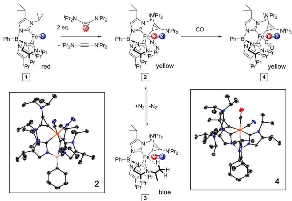
Figure 1. Synthesis of complexes. Insets show the structures of complexes 2 and 4 as determined by single crystal X-ray diffraction. Thermal ellipsoids shown at 50% probability; hydrogen atoms omitted for clarity. Black, blue, pink, and orange ellipsoids represent C, N, B, and Fe atoms, respectively.
