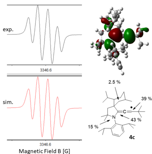
Figure 5. Experimental and simulated EPR spectra ( a_N = 4.42 G, a_H = 3.76 G) of 4c , with the SOMO and Mulliken spin densities calculated at the UB3LYP/def2-TZVP level.
