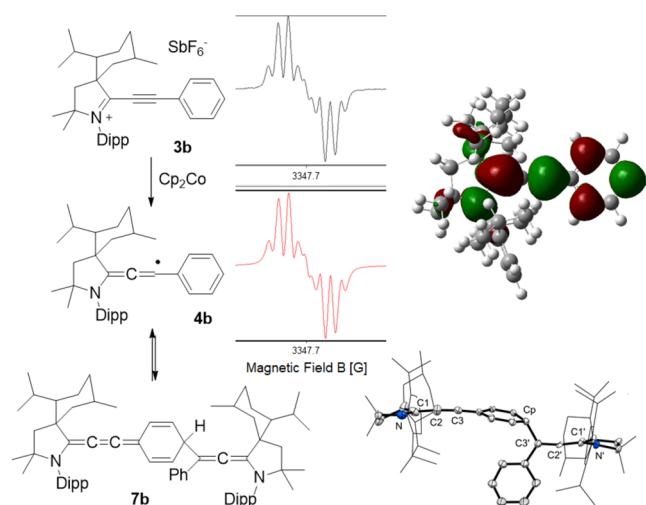
Figure 4. Synthesis of (amino)allenyl radical 4b , its experimental and simulated EPR spectra, its calculated SOMO, and the solid-state structure of its dimer 7b .
