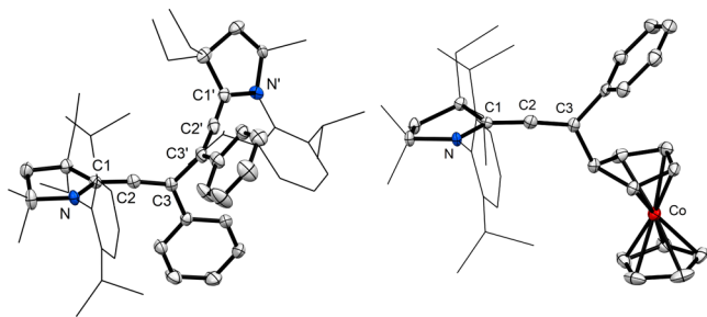
Figure 3. Solid-state structures of dimer 5a (left) and cobaltocene adduct 6a (right). Selected bond lengths [Å] and angles [°]: 5a N–C1 1.412(4); C1–C2 1.311(4); C2–C3 1.319(4); C3–C3' 1.544(4); C1–C2–C3 170.7(3); 6a N–C1 1.3947(17); C1–C2 1.3194(19); C2–C3 1.3148(19); C1–C2–C3 166.84(14).
