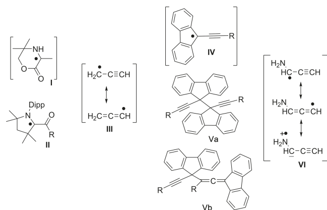
Figure 1. 2-Oxomorpholin-3-yl radical I , which dimerizes in the solid state, stable CAAC-carboxy radicals II , transient allenyl/propargyl radicals III , IV , and VI , and the isolated dimers Va and Vb .
