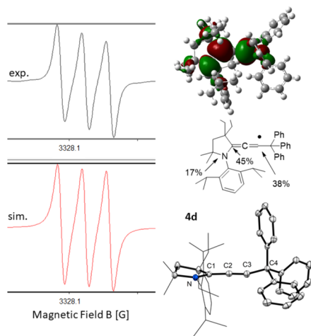
Figure 6. Experimental and simulated EPR spectra ( a_N = 4.45 G), SOMO and Mulliken spin densities calculated at the UB3LYP/def2-TZVP level, and solid-state structure of 4d . Selected bond lengths [Å] and angles [°]: N–C1 1.3850(14); C1–C2 1.3821(17); C2–C3 1.2191(17); C3–C4 1.4847(18); C1–C2–C3 177.7(12); C2–C3–C4 163.37(12).
