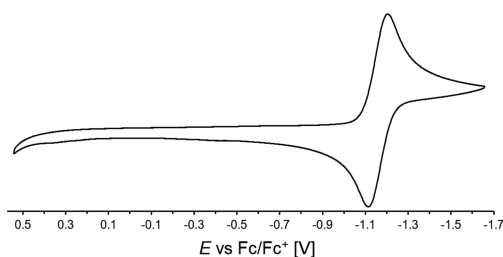
Figure 2. Cyclic voltammogram of alkynyl-iminium salt 3a . ( n\text{Bu}_4\text{NPF}_6 0.1 M in THF, 100 \text{mV s}^{-1} , vs \text{Fc}^+/\text{Fc} ).
