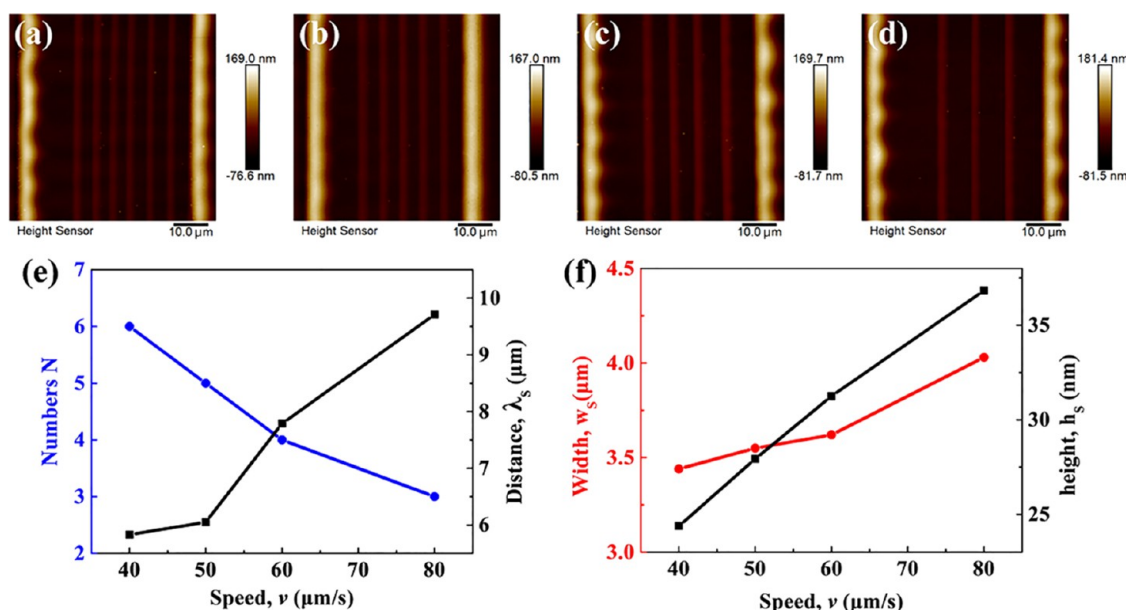
Figure 4. (a–d) AFM images of hierarchical stripes formed by FESA of PM 6 ABOC 2 toluene solution ( c = 2 mg/mL) at different moving speeds of the lower Si substrate mounted on a translational stage v . (a) v = 40 μm/s, (b) v = 50 μm/s, (c) v = 60 μm/s, and (d) v = 80 μm/s. (e) Influence of moving speed on the number of secondary stripes ( N ) within two primary stripes ( \lambda_p = 50 μm) and characteristic distance between two adjacent secondary stripes ( \lambda_s ). As the moving speed v increased from 40–50 to 60–80 μm/s, N decreased from 6–5 to 4–3, \lambda_s increased from 5.83–6.05 to 7.79–9.71 μm. (f) The lateral dimension change of each secondary stripe when altering the moving speed of the lower Si substrate. Both width w_s increased from 3.44–3.55 to 3.62–4.03 μm and height h_s increased from 24–28 to 31–37 nm, as the moving speed of the lower Si substrate increased.
