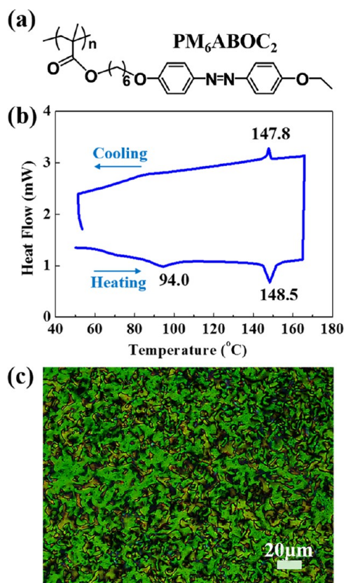
Figure 1. Structure and liquid crystalline property of the liquid crystal polymer (LCP). (a) Chemical structure of poly(6-(4-(4-ethoxyphenylazo)phenoxy)-hexyl methacrylate) ( \text{PM}_6\text{ABOC}_2 ). (b) Differential scanning calorimetry (DSC) curves of first time cooling and second time heating processes. Upon heating, an LC region ranging from 94 to 148.5 °C is clearly evident. (c) Typical schlieren texture under the polarized optical microscope (POM) at 140 °C.
