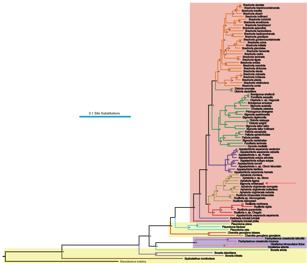
Figure 2 Molecular phylogeny of Xystodesmidae. Asterisks indicate a posterior probability of >0.70. Colored boxes indicate tribes: yellow, Rhysodesmini; purple, Pachydesmini; red, Apheloriini. Color branches and names indicate monophyletic groups that potentially warrant unique generic status: black, Stenodesmus ; brown, Gyalostethus ; light purple, Boraria ; light green, Boraria stricta ; peach, Dicellarius ; pink, Pachydesmus ; burnt sienna, Cherokia ; turquoise, Pleuroloma ; dark purple, Deltotaria brimleii philia ; blue, Deltotaria brimleii brimleii ; red, Rudiloria ; gold, Apheloria ; navy, Appalachioria ; green, sigmoid clade; mustard, Dixioria ; orange, Brachoria . The placement of Sigmoria whiteheadi within the Apheloria is indicated by a red arrow.
