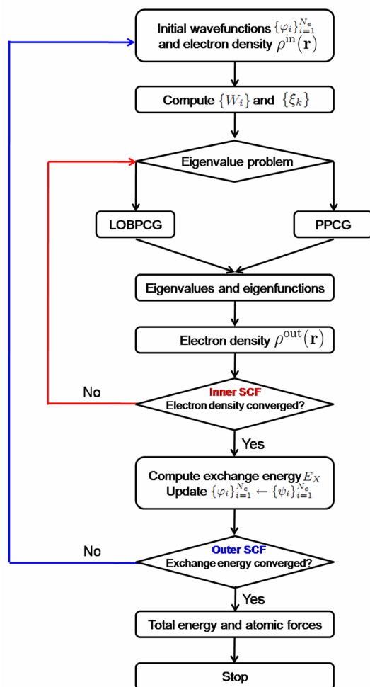
Figure 2. Flowchart of the ACE formulation for hybrid density functional calculations. The inner SCF iteration replaces the exchange operator V_X by the low rank operator V_X^{\text{ACE}} , and V_X^{\text{ACE}} is only updated at the beginning of each outer SCF iteration.
