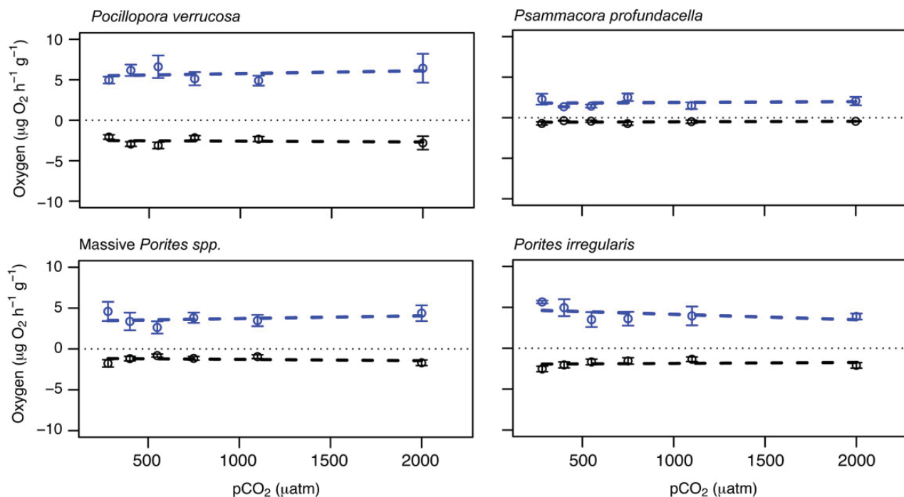
Figure 3. Biomass-normalized light respiration (black lines) and gross photosynthesis (blue lines) in corals as a function of p\text{CO}_2 . The points correspond to the mean rates at each tested p\text{CO}_2 ( n = 4 ) and the vertical bars show \pm SE. The solid line shows a significant p -value for the slope and dashed lines indicate a non-significant p -value for the slope. This figure is available in black and white in print and in colour at ICES Journal of Marine Science online.
