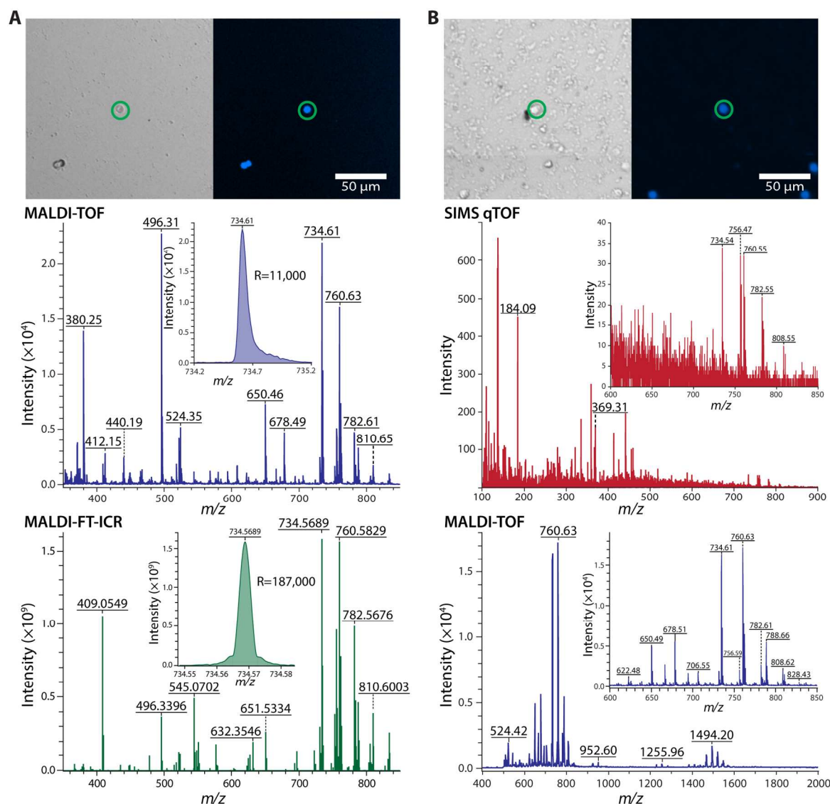
Figure 2. Sequential analysis of the same individual cell with two separate MS systems. Once a cell has been located in the optical image (top), its location remains fixed through multiple analyses, allowing two instruments to probe the same set of selected cells. (A) MALDI-TOF MS (middle) of a rat cerebellum-derived cell followed by MALDI-FT-ICR MS (bottom). MALDI-TOF MS provides high throughput screening of thousands of cells to highlight rare or representative individuals. Here, FT-ICR MS provides high mass resolution and high mass accuracy for unequivocal elemental composition of selected cellular contents. (B) SIMS profiling (middle) followed by MALDI-TOF MS (bottom) with a DHB-coated, SCN-derived cell. SIMS provides information on small molecule compounds while MALDI-TOF MS effectively detects larger species, such as lipid dimers and peptides. The insets demonstrate overlap of intact lipid coverage from each modality. Reproduced with permission from Comi, T. J., Neumann, E. K., Do, T. D., Sweedler, J. V.: microMS: A python platform for image-guided mass spectrometry profiling . J. Am. Soc. Mass Spectrom. 28, 1919–1928 (2017) (ref. 64 ). Copyright American Society for Mass Spectrometry 2017, with permission from Springer.
