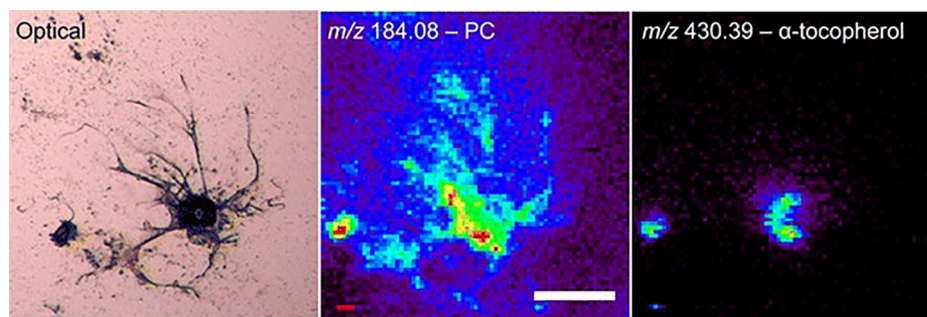
Figure 3. Distribution of metabolites in cultured A. californica buccal neurons was performed by C 60 -SIMS imaging. Cells were cultured on silicon tiles and stabilized with glycerol. C 60 -SIMS ion images revealed that phosphocholine (PC) and \alpha -tocopherol showed different locations in neurons. Cell bodies and processes are apparent in the PC image ( m/z 184.08, 0–200 counts), while \alpha -tocopherol accumulated almost exclusively within the cell bodies ( m/z 430.39, 0–50 counts). Adapted with permission from Lanni, E. J., Dunham, S. J., Nemes, P., Rubakhin, S. S., and Sweedler, J. V. (2014) Biomolecular imaging with a C60-SIMS/MALDI dual ion source hybrid mass spectrometer: Instrumentation, matrix enhancement, and single cell analysis, J. Am. Soc. Mass Spectrom. 25, 1897-1907 (ref. 72 ). Copyright 2014, American Society for Mass Spectrometry, with permission from Springer.
