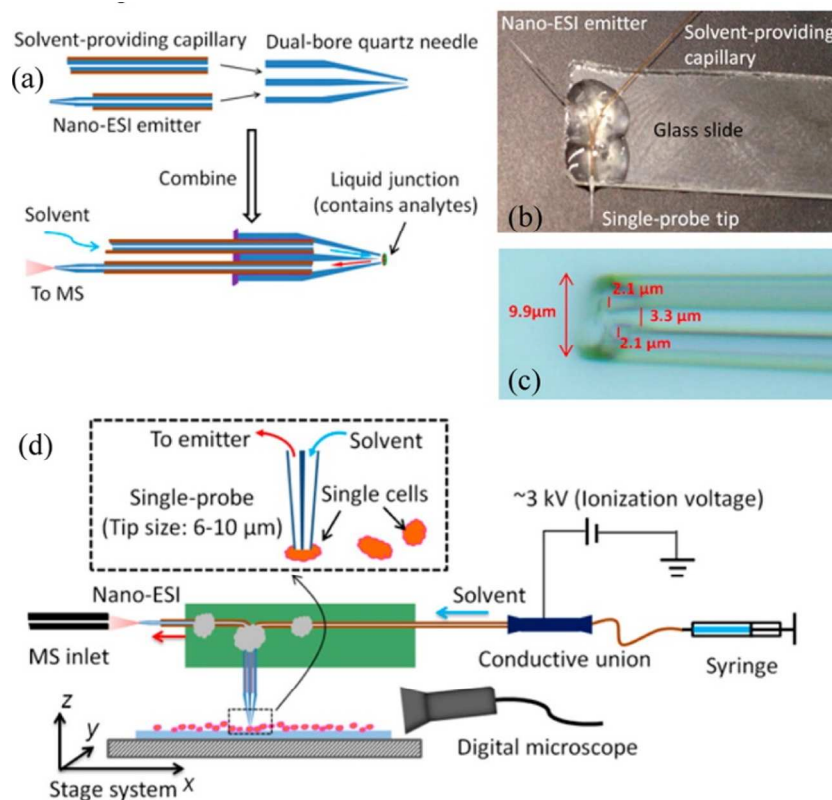
Figure 1. (a) Fabrication steps and structure of a Single-probe for ESI-MS; (b) photograph of a working Single-probe; (c) 40 \times magnification of the Single-probe tip with measurements obtained from the calibrated digital microscope; (d) setup schematic of an in situ real-time single cell MS analysis. Reproduced with permission from Pan, N., Rao, W., Kothapalli, N. R., Liu, R., Burgett, A. W. G., and Yang, Z. (2014) The single-probe: A miniaturized multifunctional device for single cell mass spectrometry analysis, Anal. Chem. 86, 9376-9380 (ref. 48 ). Copyright 2014, American Chemical Society.
