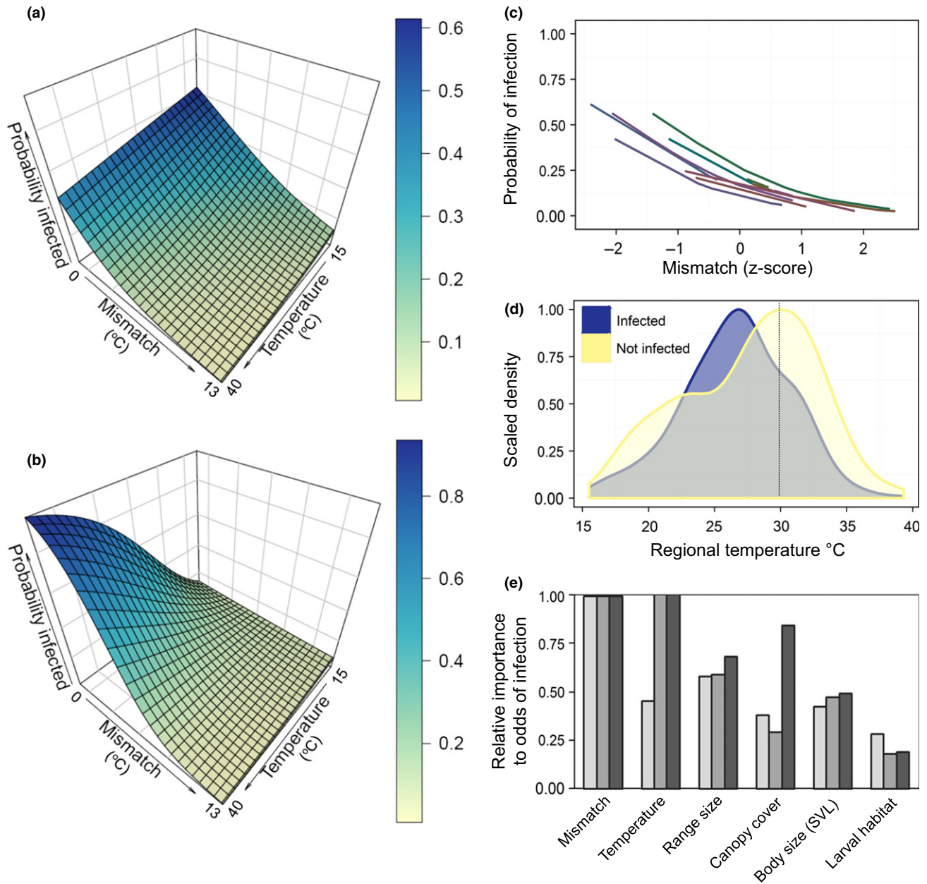
Figure 3 Effects of thermal tolerance mismatch and environmental context on infection risk from a global-scale analysis. Predicted probability of Batrachochytrium dendrobatidis (Bd) infection as a function of thermal tolerance mismatch ('Mismatch') and mean maximum temperature of the warmest month ('Temperature') in areas with low (a; 30%) and high (b; 90%) canopy cover. Thermal tolerance mismatch was calculated as the difference between the amphibian host's and Bd's upper thermal limits. Estimates were generated from a generalised linear mixed model (an aggregated binomial regression) that included the interactions among three predictor variables: thermal tolerance mismatch, regional temperature and canopy cover (model 'Tolerance mismatch B' in Table S1). The model included varying intercepts among studies and among species nested within families. (c) Predicted probability of infection in relation to thermal tolerance mismatch for different amphibian families included as varying intercepts. (d) Density plot of mean maximum temperature of the warmest month grouped by infected and non-infected records from Bd-Maps (vertical line represents upper thermal limit for Bd growth in culture; Piotrowski et al. 2004). (e) The relative variable importance to the odds of infection calculated as cumulative Akaike weights of models containing each variable from all possible additive models. Separate bars are shown for model sets that included mean maximum temperature of the warmest month (light grey), mean annual temperature (medium grey), or the standard deviation of monthly maximum temperatures (dark grey).
