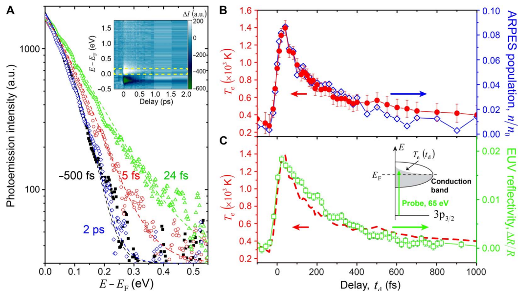
Fig. 3. Ultrafast charge dynamics in Ni. (A) Log plots of the photoemission intensity above E_F for F \approx 6 \text{ mJ/cm}^2 and at different t_d , integrated from k_{||} \approx 0.85 \text{ \AA}^{-1} to k_{||} \approx 1.3 \text{ \AA}^{-1} in the momentum space. The dashed lines represent the fitting of the photoemission intensities with the Fermi-Dirac distribution convolved with experimental energy resolution (see the Supplementary Materials). Inset: Integrated photoemission intensity as a function of pump-probe time delay. The yellow dashed box illustrates the integration region of electron population in (B). (B) Dynamics of the electron temperature and the relative electron population ( n/n_0 ) within \sim 0.2 \text{ eV} above E_F as a function of t_d . The electron population is normalized to the band electron population ( n_0 ) \sim 0.2 \text{ eV} below E_F (see the Supplementary Materials). (C) Comparison of the electron temperature [red dashed line, same as (B)] and the change of EUV transient reflectivity at a similar pump fluence. Inset: EUV transient reflectivity measurement. The resonant EUV light (65 eV) directly probes the charge dynamics around E_F induced by the laser pump pulse. This measurement is averaged over k -space.
