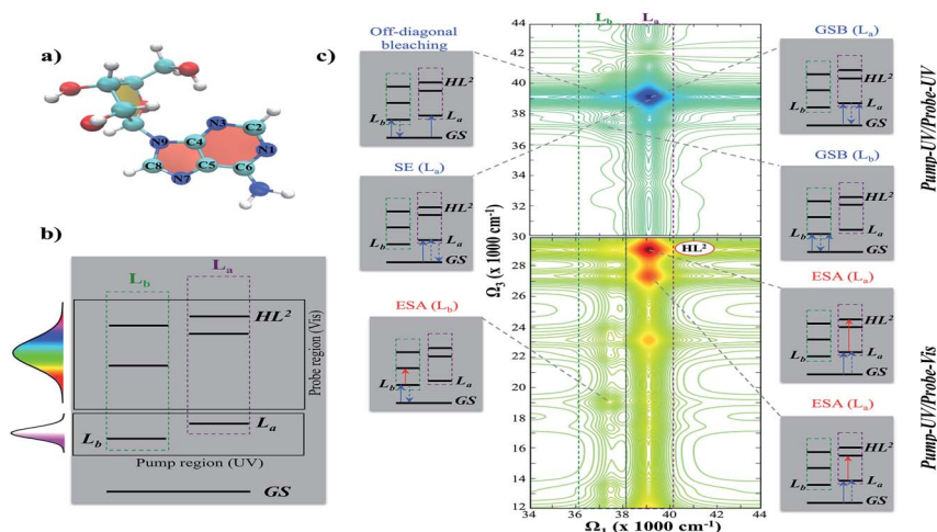
Fig. 1 2DES spectrum of adenosine monophosphate, where (a) displays the molecular system and atom labelling, (b) shows a scheme of the energy levels that are accessible with different laser pulses and (c) shows the 2DES in the Vis (lower panel) and UV (upper panel) probe windows, together with energy level schemes depicting the different signals featured in terms of the laser pulse sequence. A red colour denotes positive (ESA) signals. A blue colour denotes negative (GSB, off-diagonal bleach and SE) signals. The SE signal associated with the ^1L_b state was not included in the scheme for simplicity, being placed on top of GSB( L_b ). The signal intensity in each spectrum is normalised according to the absolute value of the most intense signal.
