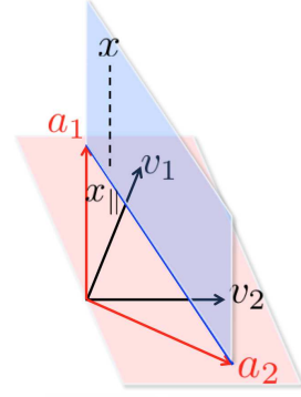
Figure 1: \mathbf{v}_1, \mathbf{v}_2 correspond to class 1 and 2, and \mathbf{a}_1 and \mathbf{a}_2 correspond to canonical vectors purely of class 1 and 2, respectively.
