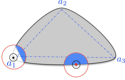
Figure 2: Demonstrating the distinction between points close to \mathbf{a}_i and far from \mathbf{a}_i . The convex hull of CH(\hat{S}_{\parallel} \setminus B_{r_2}(\hat{\mathbf{x}})) , which is a subset of the blue and gray region, intersects B_{r_1}(\hat{\mathbf{x}}) only for \hat{\mathbf{x}} that is sufficiently far from \mathbf{a}_i 's.
