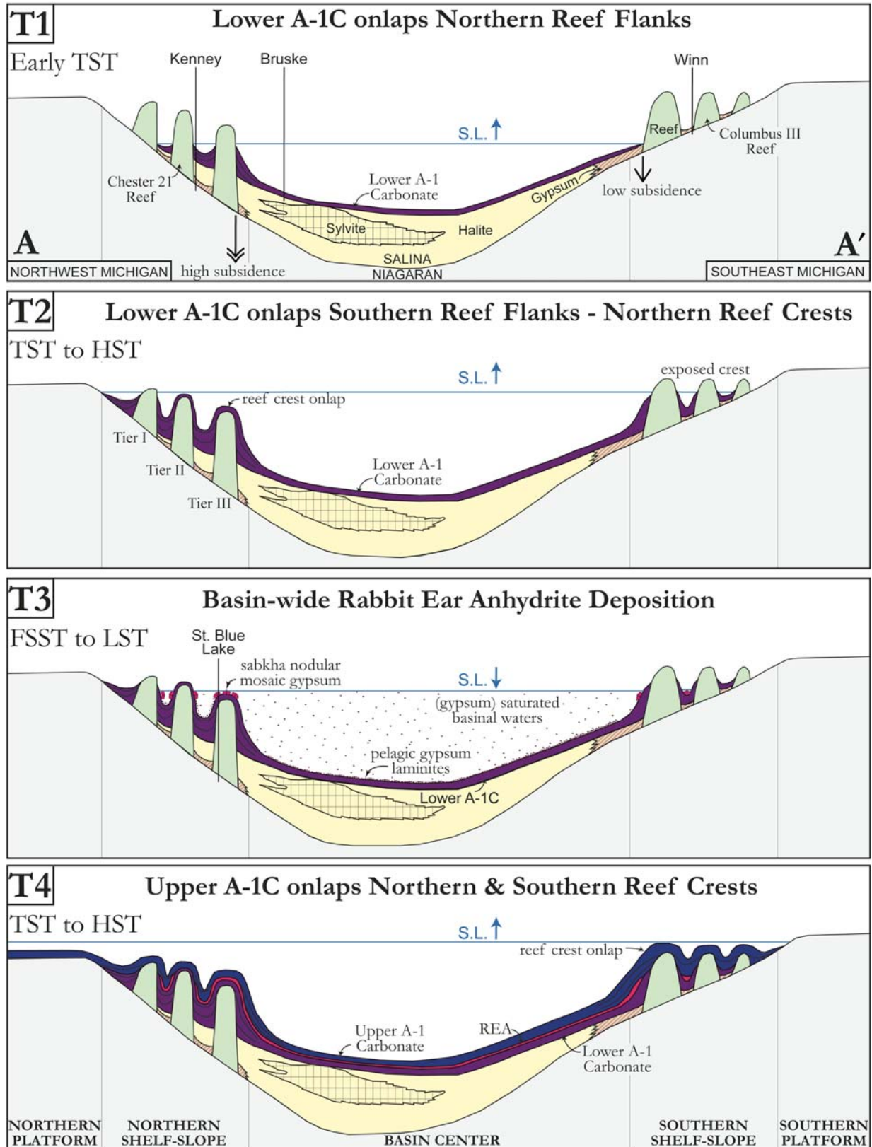
Figure 9. Generalized basinwide sequence stratigraphic model for deposition of the A-1 Carbonate (not to scale). Refer to the cross-section line A–A' on Figure 1A. SL—sea level; LST—lowstand systems tract; TST—transgressive systems tract; FSST—falling stage systems tract; HST—highstand systems tract; REA—Rabbit Ears Anhydrite.
