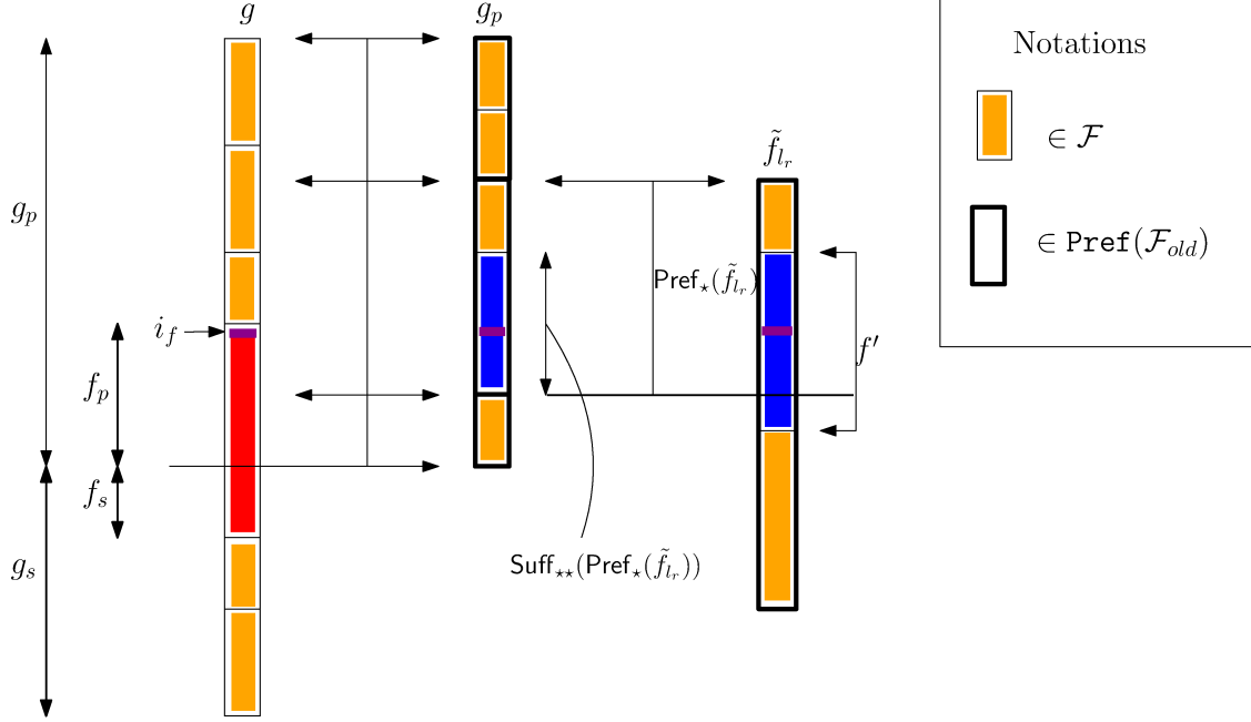
Figure 5: (f, f')^{(2)} -type failure where i_f \in_{\text{d1}} \text{Suff}_*(\text{Pref}_*(\tilde{f}_{l_r}))
