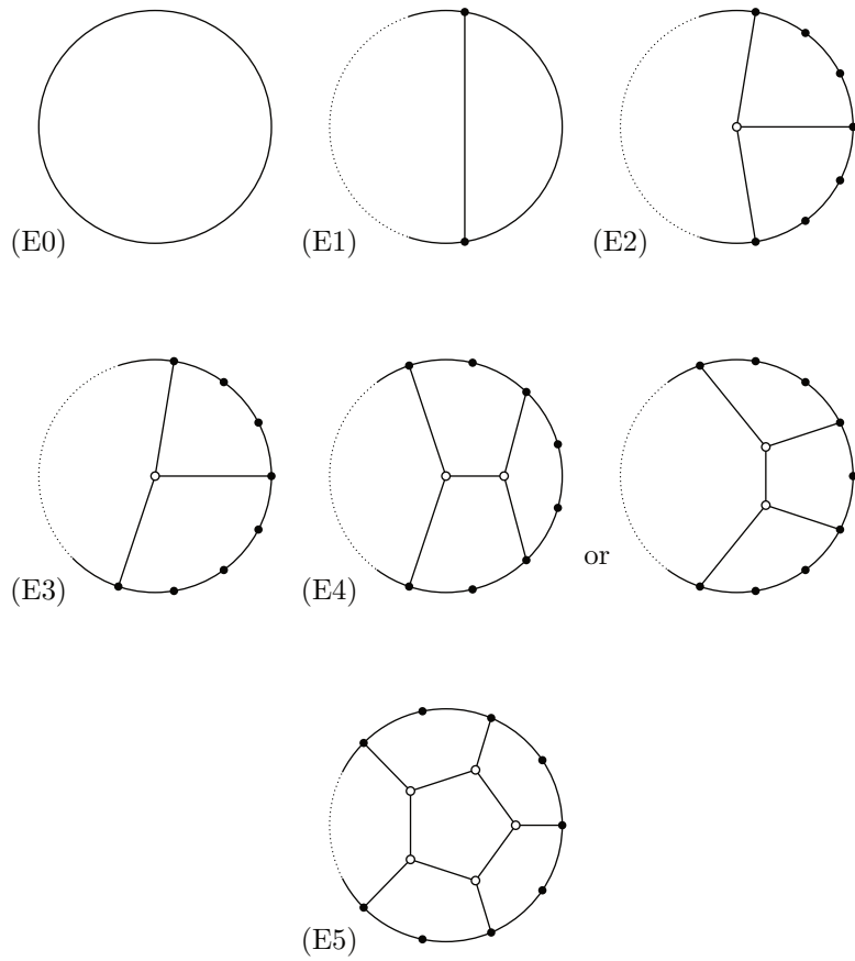
Figure 4: Exceptional graphs.
