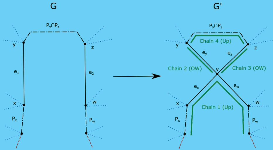
FIG. 2. An illustration of the procedure in Claim 1. The original up chain J_1 = J_2 is on the left, while its replacements in G' are on the right. The red/dashed edges are in earlier chains than J_1 = J_2 , while the blue/dotted edges are in later chains than J_1 = J_2 . The black/dashed-and-dotted segments represent paths which may have any length (including 0).
