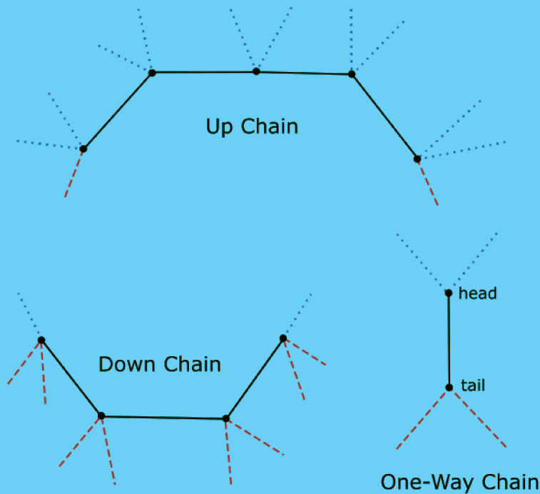
FIG. 1. An illustration of an up chain of length 4, a down chain of length 3, and a one-way chain. The red/dashed edges are in earlier chains, while the blue/dotted edges are in later chains.
