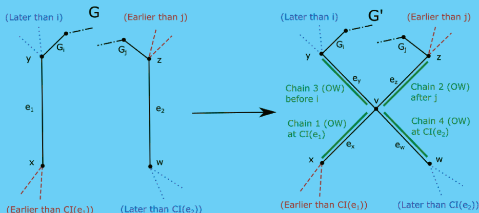
FIG. 4. An illustration of the procedure in Claim 5. The original chains J_1 and J_2 are on the left, while their replacements in G' are on the right. The red/dashed edges are in earlier chains, while the blue/dotted edges are in later chains, with the particular meanings of “earlier” and “later” in the corresponding labels. The black/dashed-and-dotted segments represent paths which may have any length (including 0).
