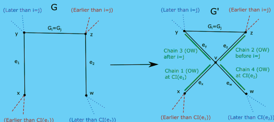
FIG. 3. An illustration of the procedure in Claim 4. The original chains J_1 and J_2 are on the left, while their replacements in G' are on the right. The red/dashed edges are in earlier chains, while the blue/dotted edges are in later chains, with the particular meanings of “earlier” and “later” in the corresponding labels.
