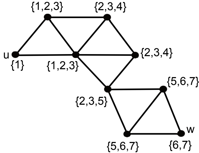
Figure 1: A coloring harmonica from u to w .
