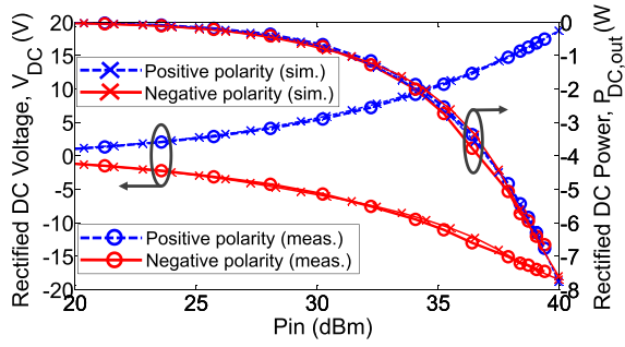
Fig. 4. Measurement and simulation results of rectified dc voltage and power for R_{dc} = 45 \Omega , and gate bias condition of V_{GG,RP} = -3.3 V and V_{GG,RN} = -5.2 V.
