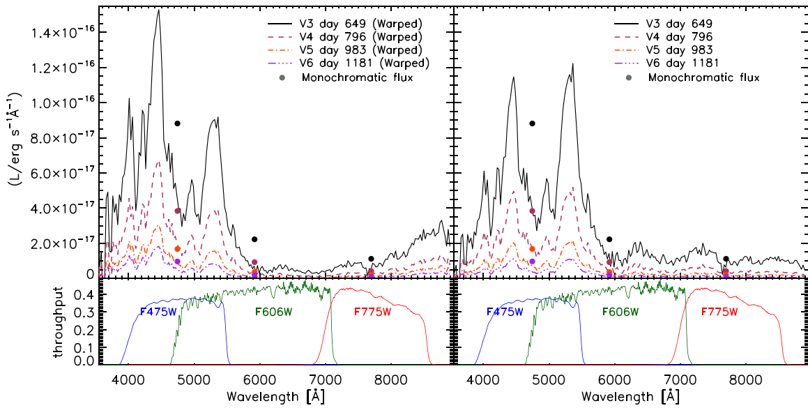
Figure 2. Constructed late-time SED for SN 2014J. The dots show the bandpass monochromatic flux from HST observations at their effective wavelengths. The solid, dashed, dashed-dotted, and triple-dotted-dashed lines show the spectra constructed with the warping procedure (left panel) and with grayscaling (right panel) as described in Section 3, from V3 to V6, respectively. The lower panels present the total bandpass throughput curve ( HST + ACS) for our F475W , F606W , and F775W observations, showing the spectral response corresponding to the monochromatic fluxes calculated from the observed photometry.
