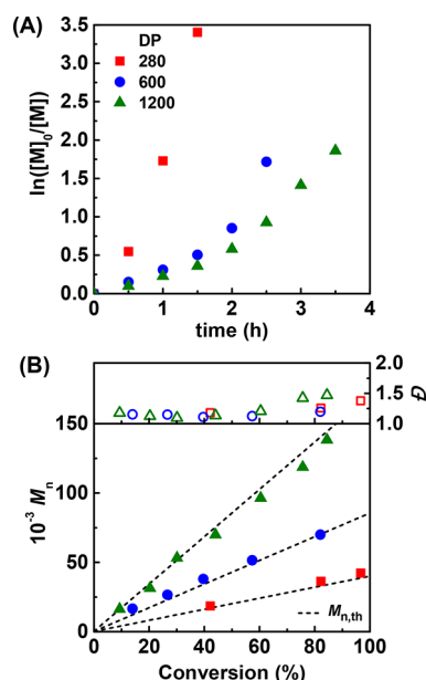
Figure 3. Miniemulsion ARGET of BMA with different target D with different target DPs (280, 600 and 1200). (A) Kinetic plot and (B) MW and D vs monomer conversion. [AsAc]/[Cu^{II}] = 0.5 . Other reaction conditions listed in Table 1.
