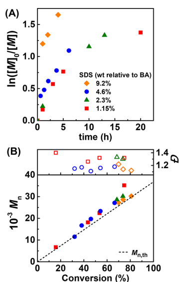
Figure 1. ARGET miniemulsion ATRP of BA with different amounts of SDS (Table 3). (A) Semilogarithmic kinetic plot and (B) MW and Đ evolution vs conversion. [AsAc]/[Cu II ] = 0.5 added dropwise at t = 0 h. Other conditions as in Table 1.
