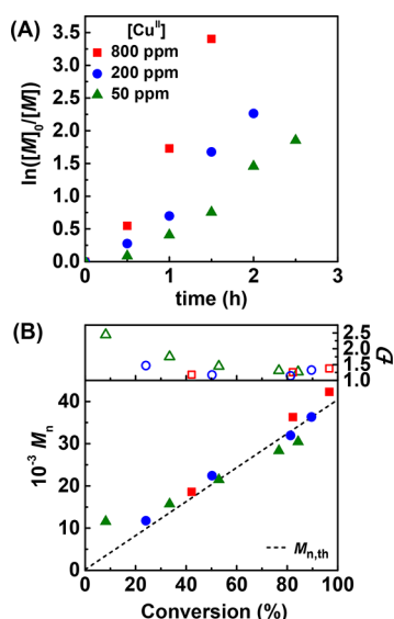
Figure 2. Miniemulsion ARGET ATRP of BMA with various catalyst loadings. (A) Semilogarithmic kinetic plot and (B) MW and \bar{D} evolution vs monomer conversion. [AsAc]/[Cu II ] = 0.4, injected dropwise every 30 min. Other reaction conditions are listed in Table 1.
